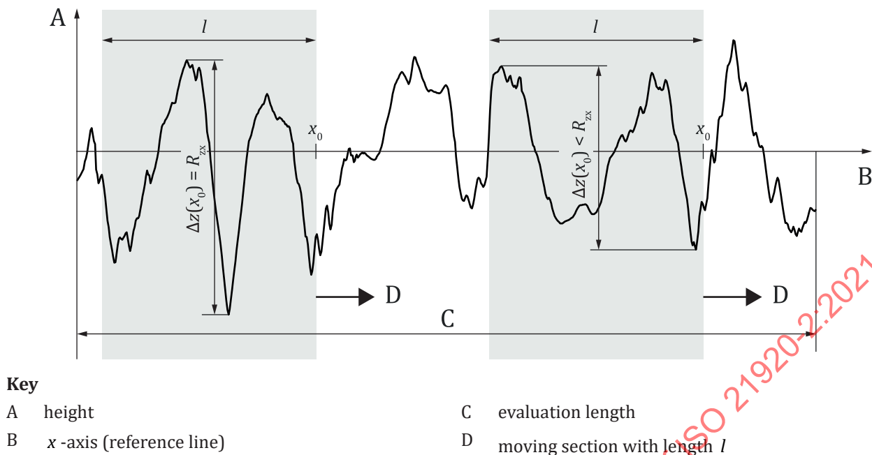
Figure 18 — Maximum height per section
