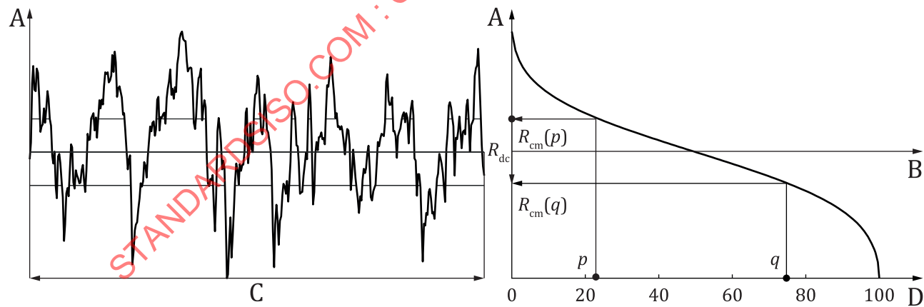
Key A height C evaluation length B x-axis (reference line) D material ratio expressed as a percentage
