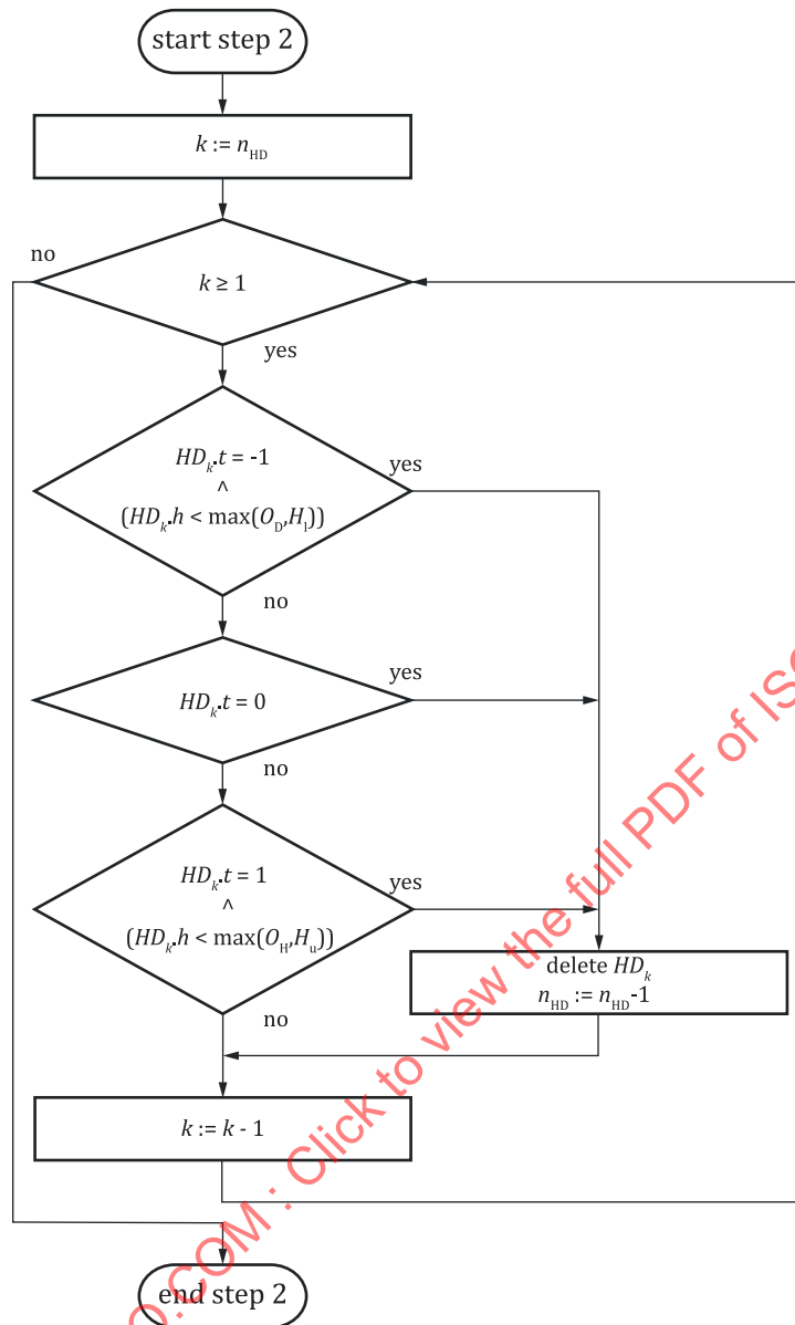
Figure E.2 — Step 2: Determination of significant profile hills and profile dales
