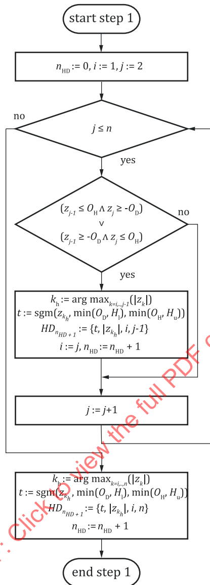
Figure E.1 — Step 1: Determination of hills and dales within the evaluation length
