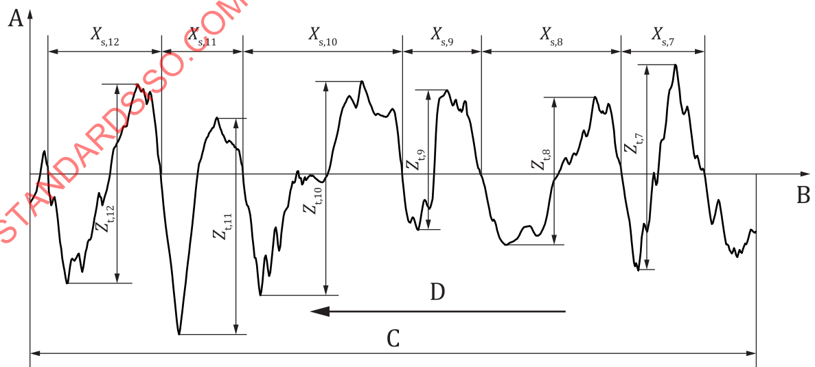
Figure 31 — Determination of profile elements from the beginning to the end
