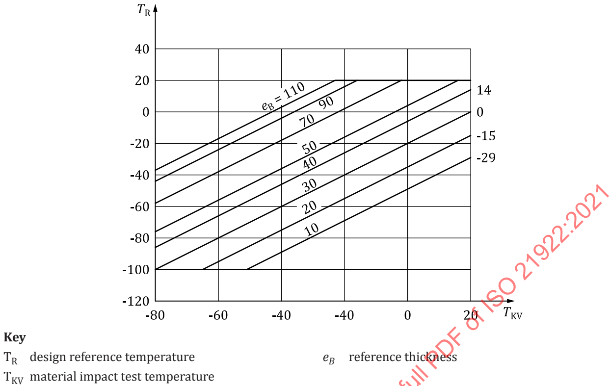
Figure D.5 — Design reference temperature and impact test temperature, post weld heat treated (PWHT) condition, for R_e \leq 460 MPa and KV \geq 40 J
