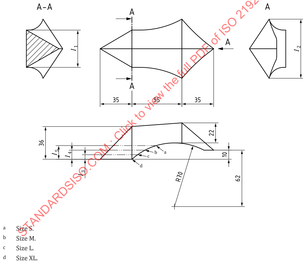
Figure 2 — Minimum volume protected by the genital protectors for males
