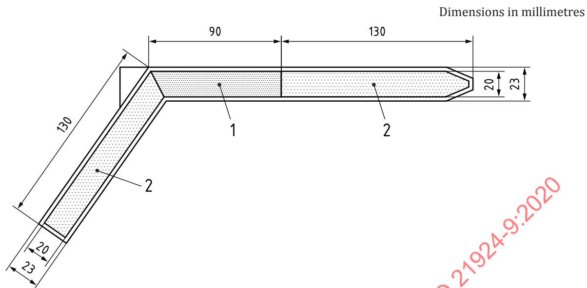
a) outside view of the locking strap
