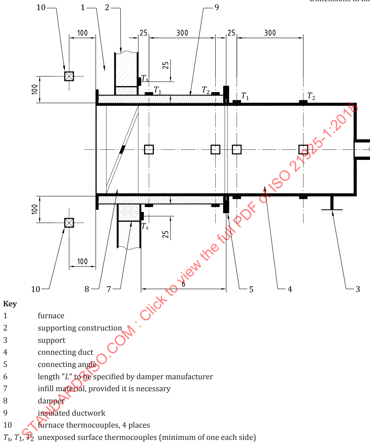
Figure 3 — Position of surface thermocouples when damper is installed in an insulated duct
