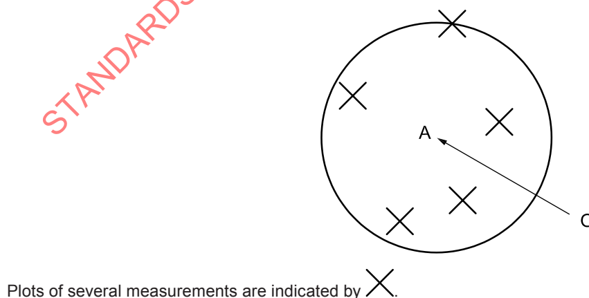
Figure 2 — Plot of measured vectors of residual unbalance or vibration (randomly variable errors)
