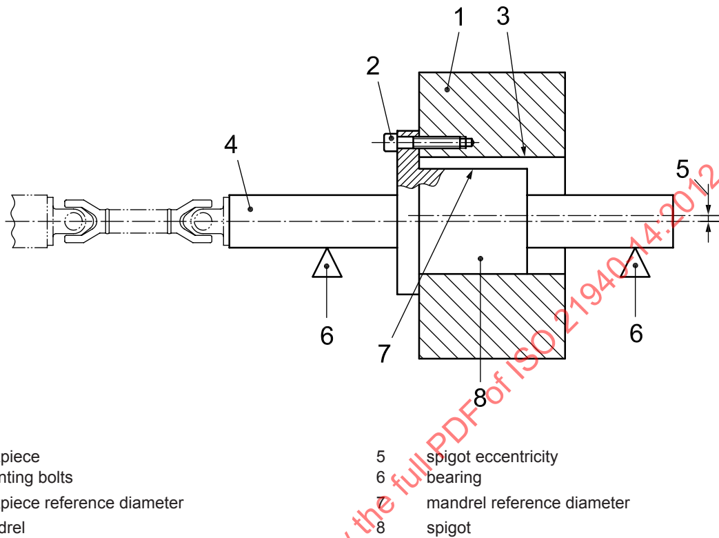
Figure A.1 — Workpiece located on mandrel
