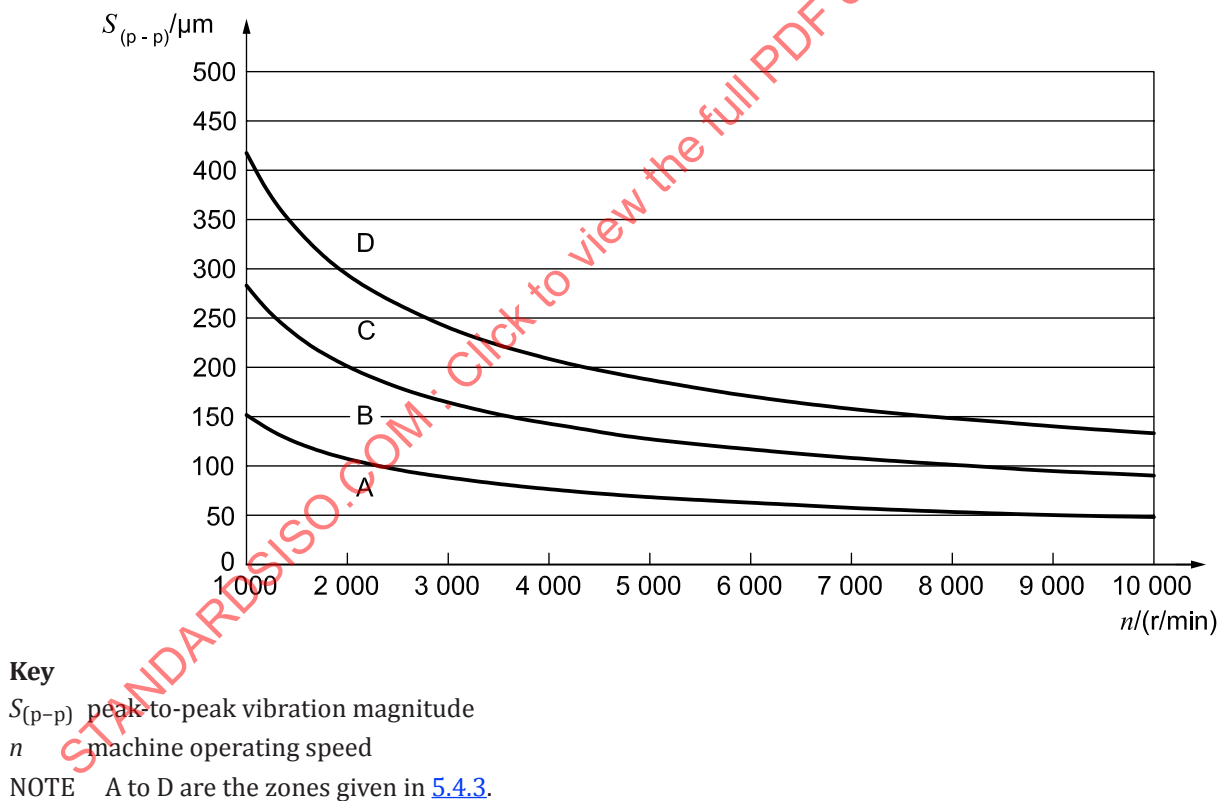
Figure 2 — Zone boundary curves according to ISO 7919-2[2] and ISO 7919-4[3]
