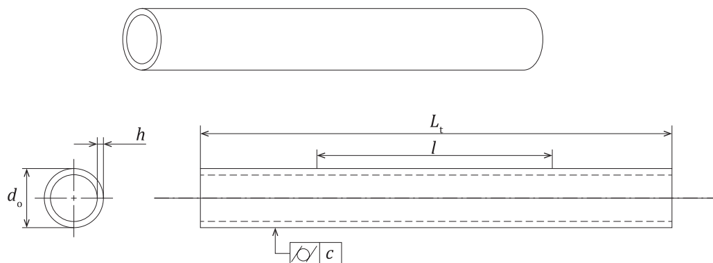
Figure 3 — Straight-sided tube test specimen
