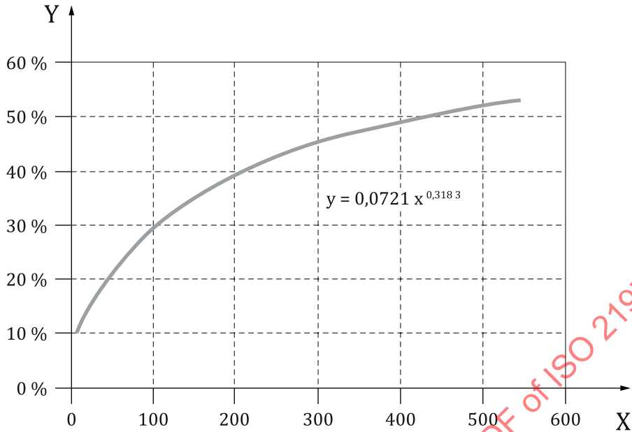
a) Efficiency of circulating pumps with a hydraulic power lower than or equal to 500 W (source: COSTIC)
