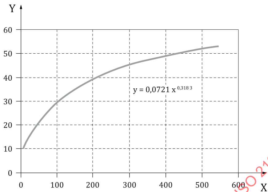
a) Efficiency of circulating pumps with a hydraulic power lower than or equal to 500 W (source: COSTIC)
