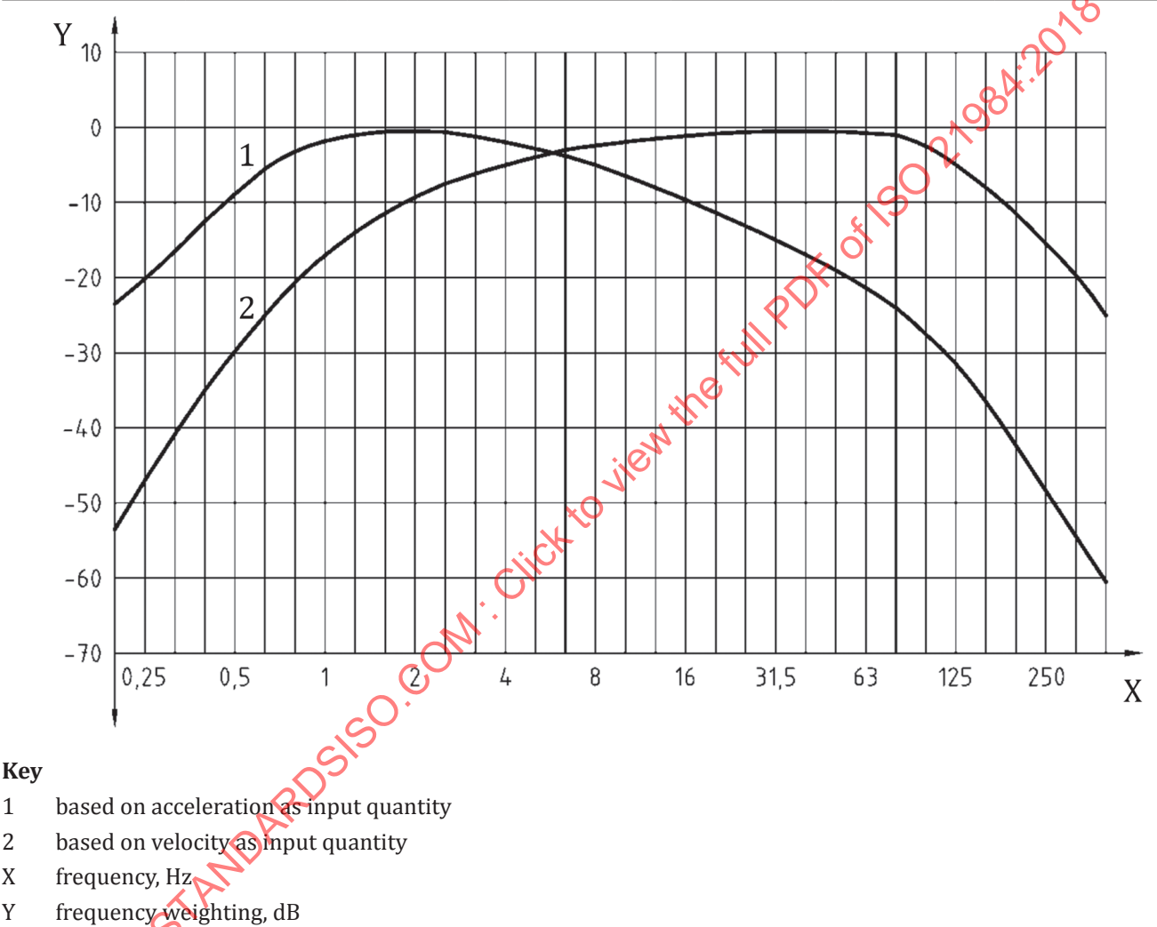
Figure B.1 — Frequency weighting curve, W_m , band limitation included (schematic)
