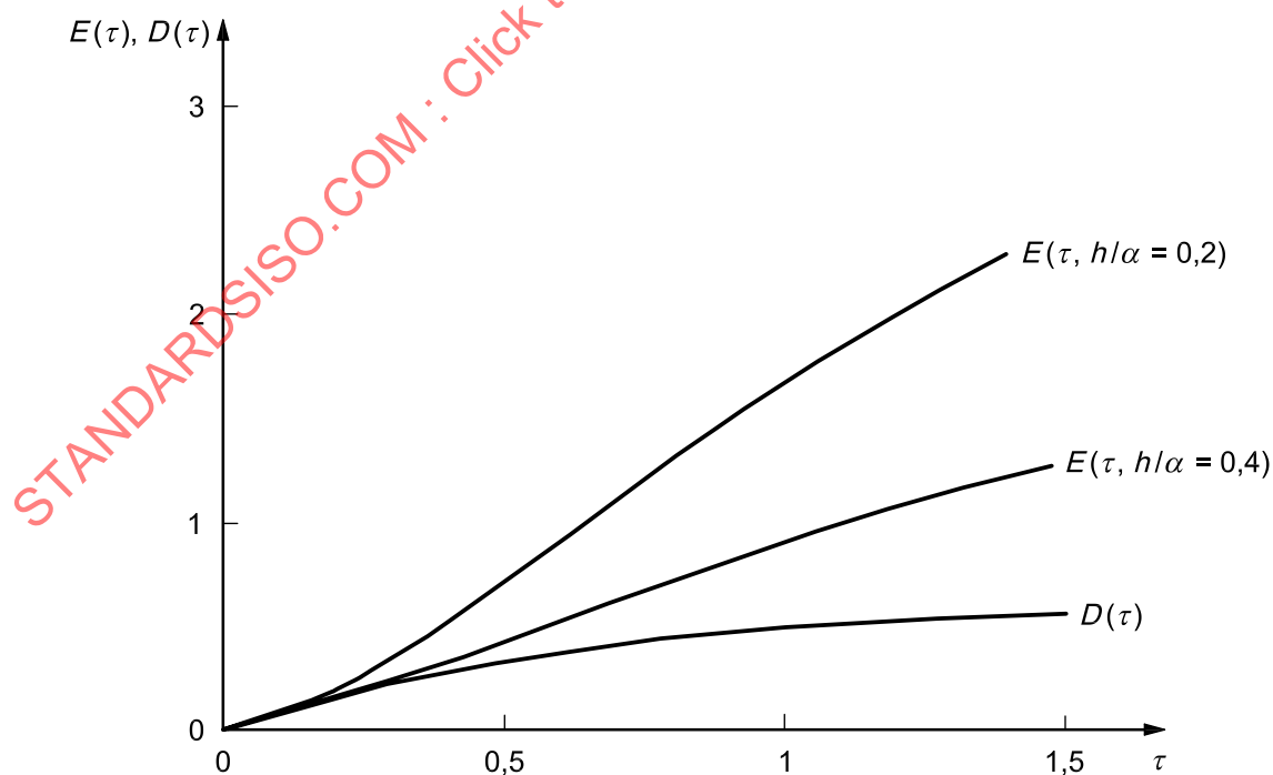
Figure 5 — D(\tau) and E(\tau) functions plotted for values of \tau up to 1,5 (In all three cases, it has been assumed that the number of concentric ring sources is 10.)
