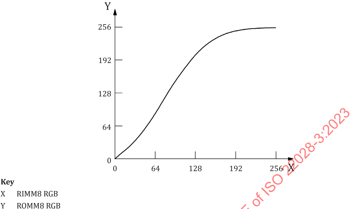
Figure A.1 — Example tone scale LUT for colour rendering scene-referred RIMM8 RGB colour space encoding values to output-referred ROMM8 RGB colour space encoding value
