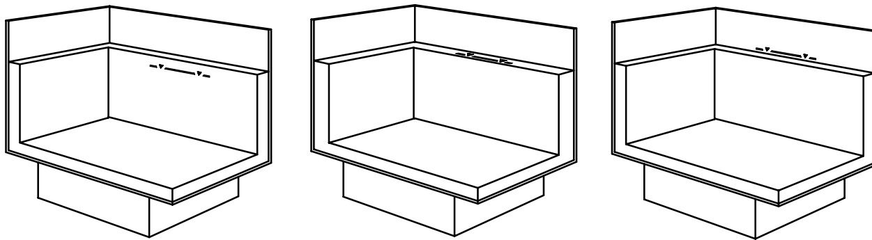
Figure 17 — Different positions for the load limit
