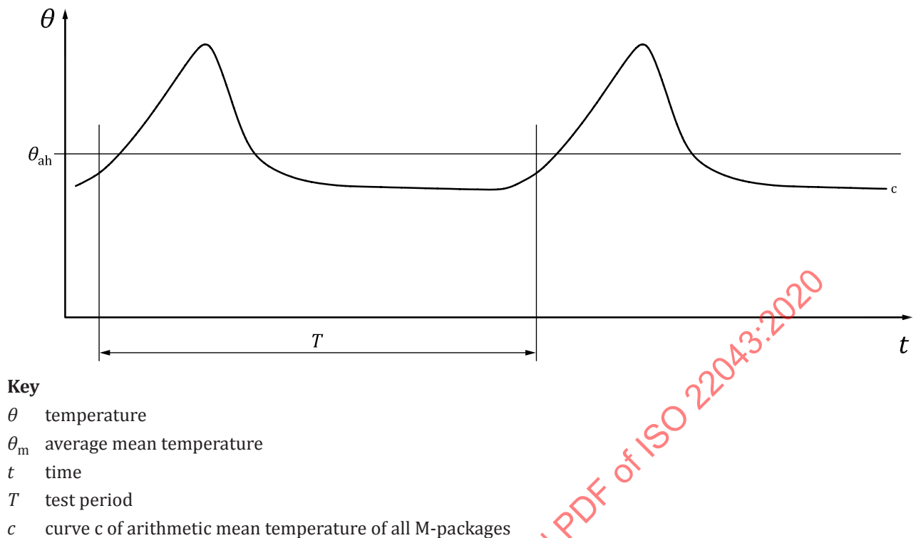
Figure 13 — Arithmetic mean temperature of M-packages
