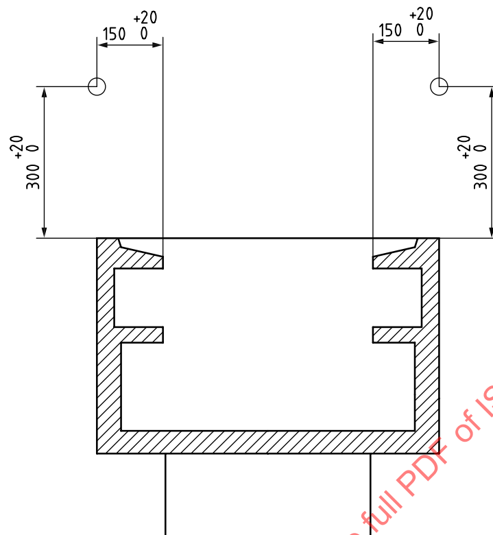
Figure 8 — Climate measuring point for ice-cream freezer
