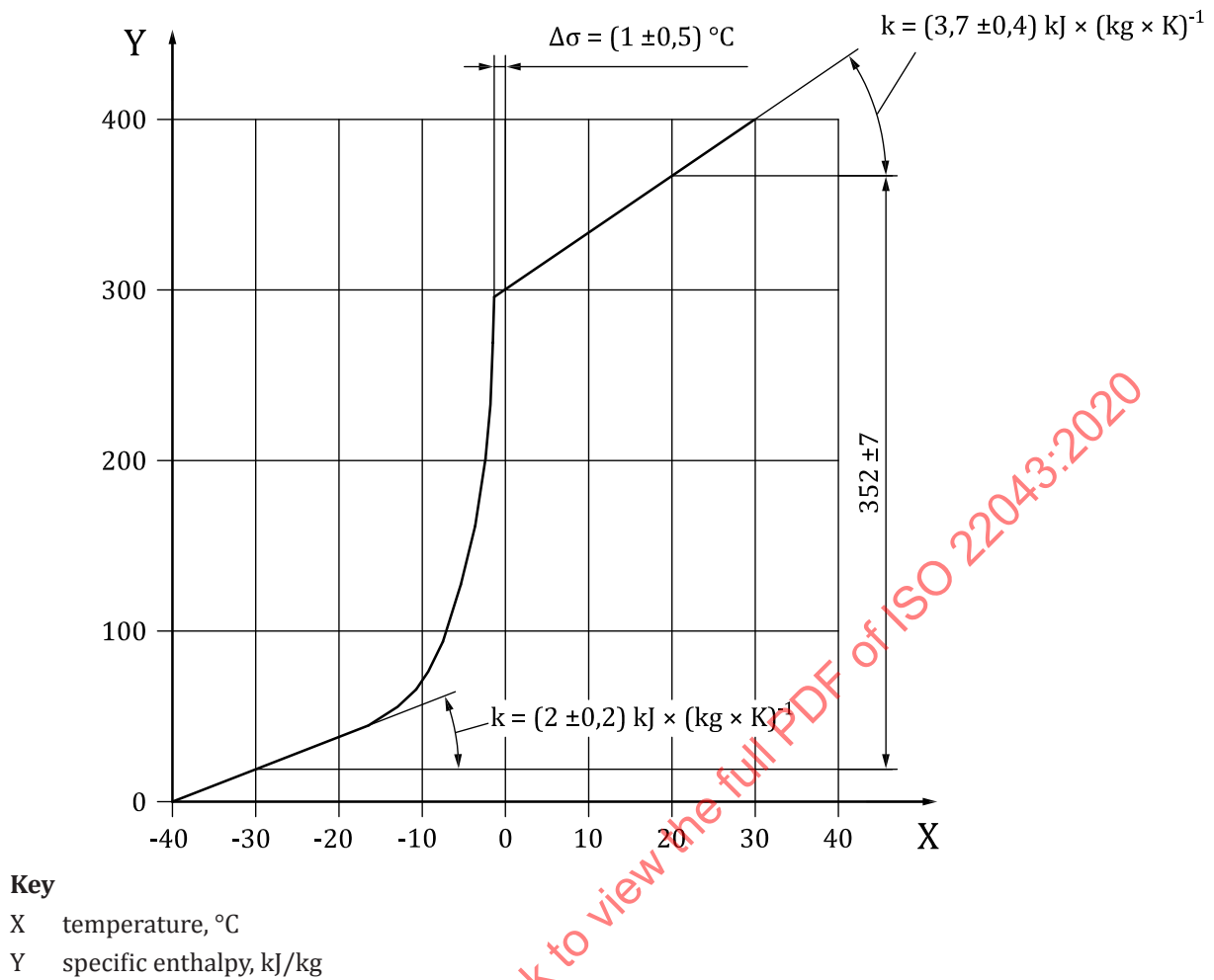
Figure 2 — Thermal characteristics of test packages
