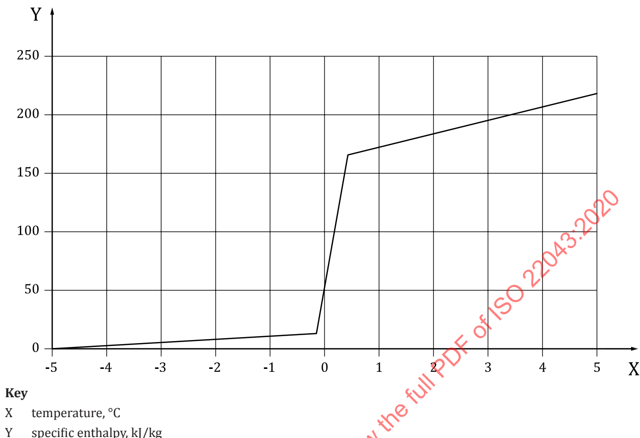
Figure 4 — Thermal characteristics of filler packages
