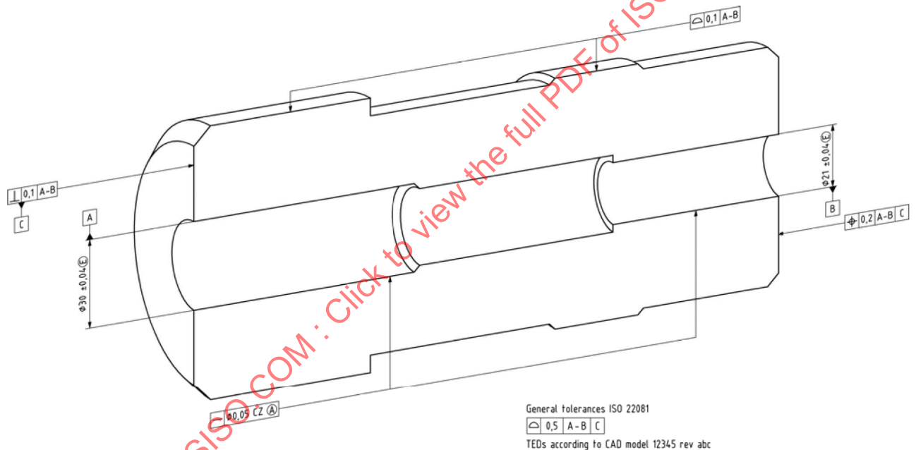
Figure B.2 — Example with two datums in the datum system of the general geometrical specification
