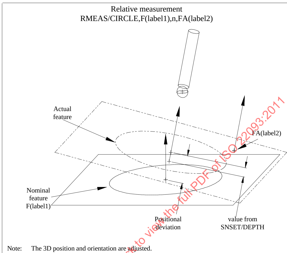
Figure B.53 — RMEAS/CIRCLE with FA(lname2)
