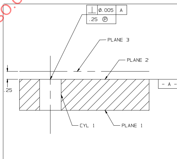
Figure 4 — Boundaries applied to a feature and tolerance
