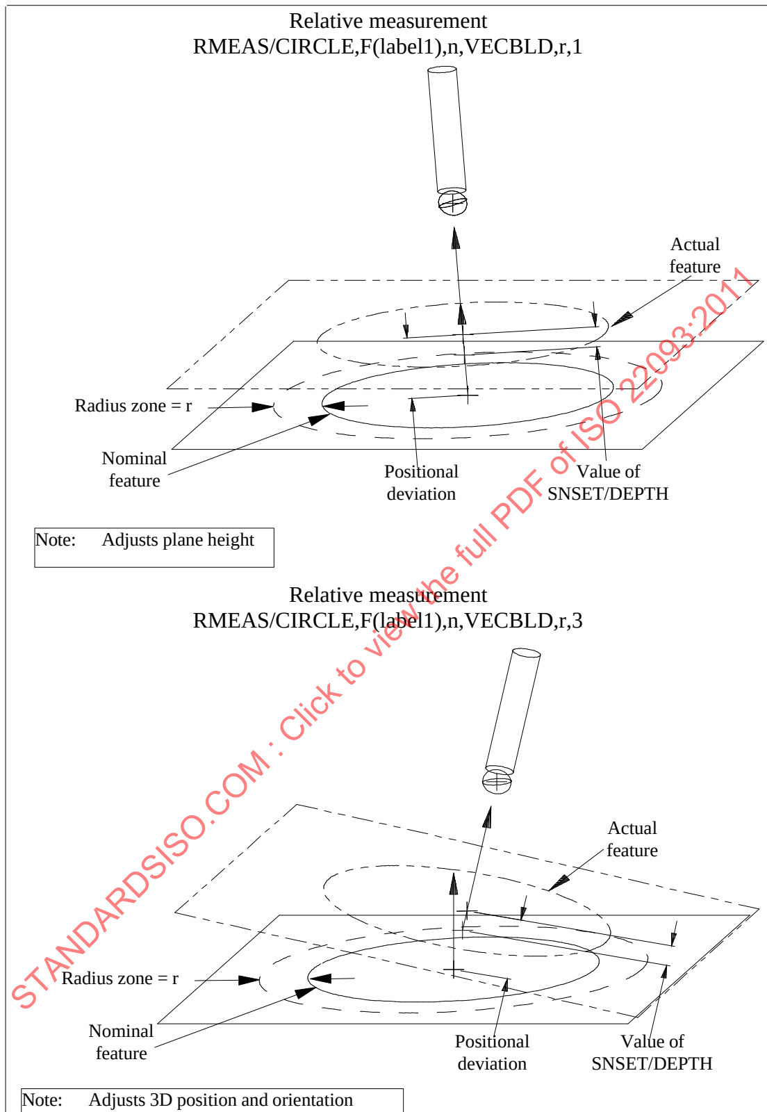
Figure B.54 — RMEAS/CIRCLE with VECBLD,r,1 and with VECBLD,r,3
