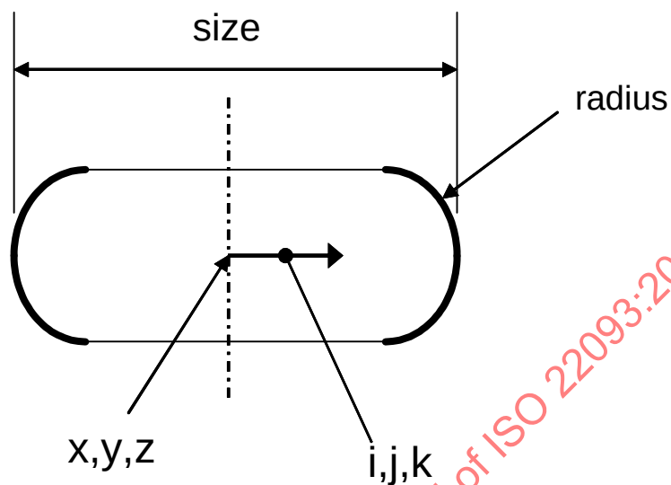
Figure B.40 — An elongated cylinder feature
