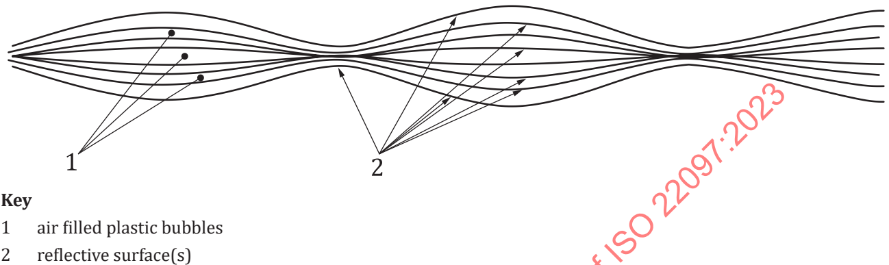
Figure 3 — Example of stitched multi-foil insulation
