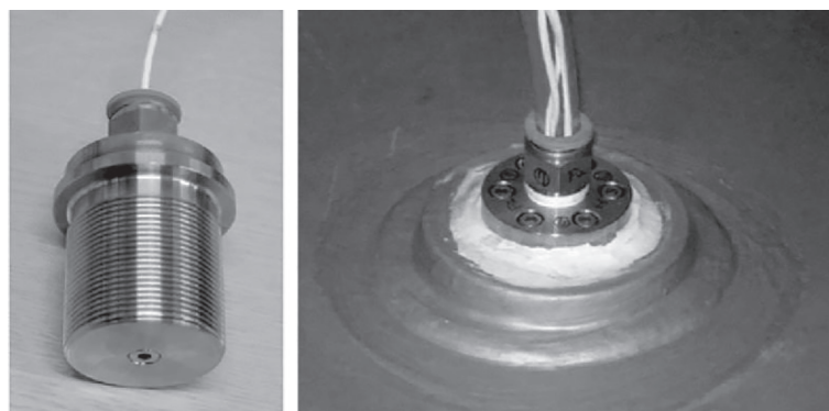
Figure 3 — Example of pressure transducers as mounted
