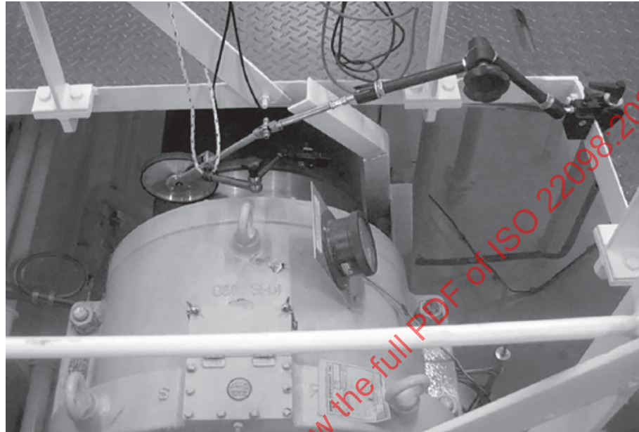
Figure 5 — Example of a pulse generator installed on a propeller shaft
