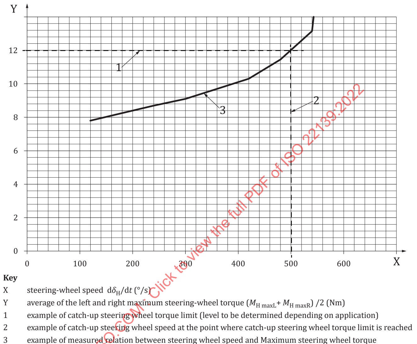
Figure 3 — Maximum steering-wheel torque vs. steering-wheel speed
