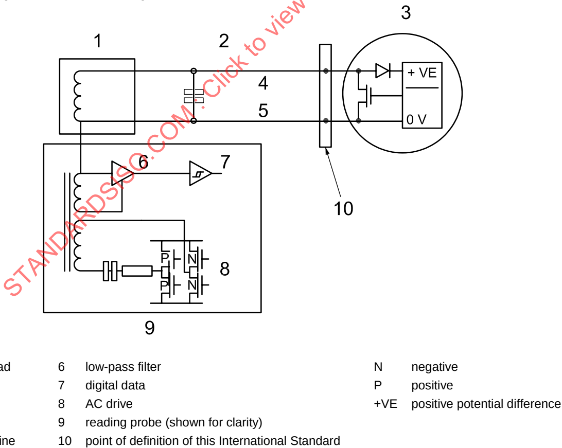
Figure 6 — Typical configuration for non-addressable two-wire asynchronous mode for reading via an inductive pad and probe
