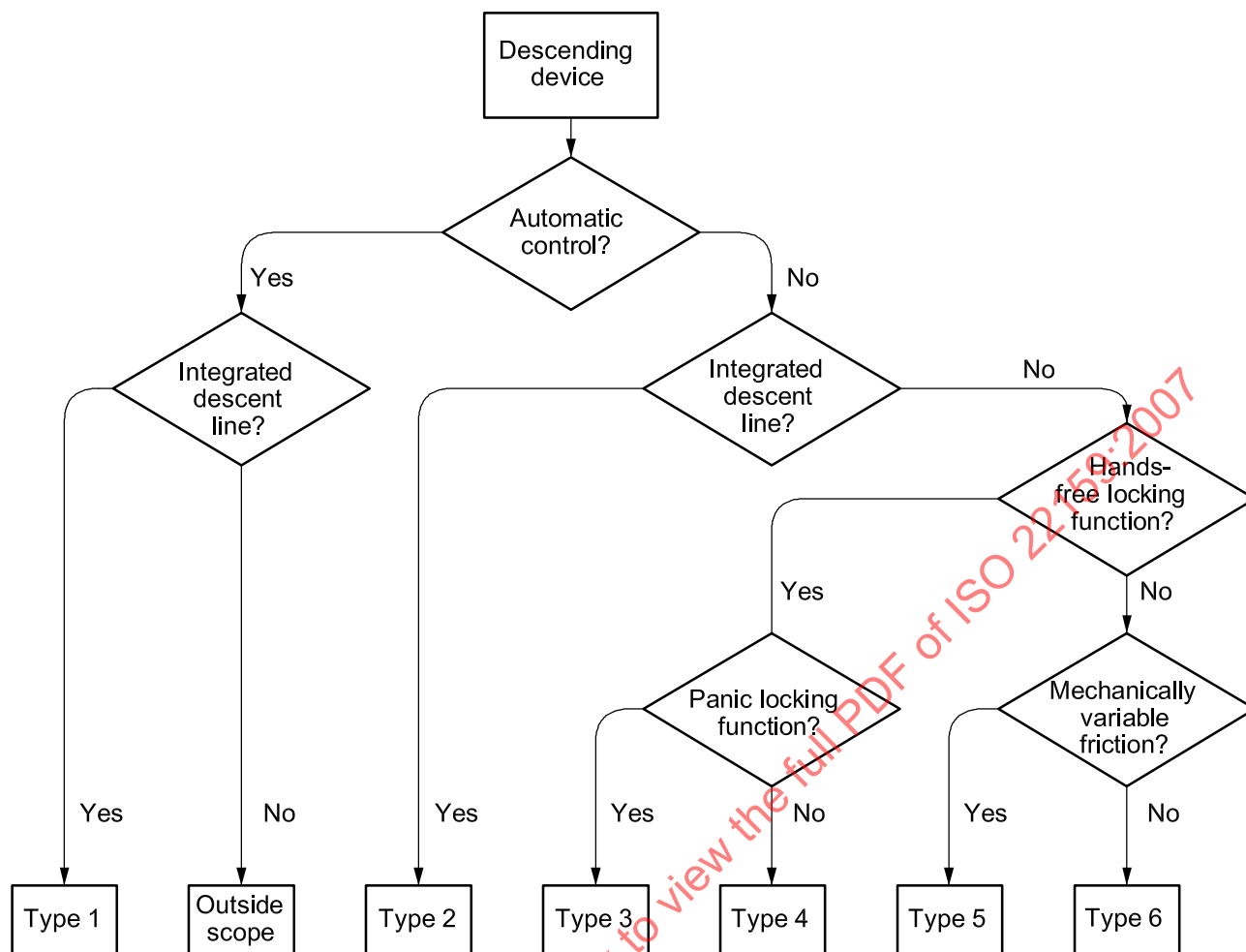
Figure 2 — Characteristics of different types of descending device
