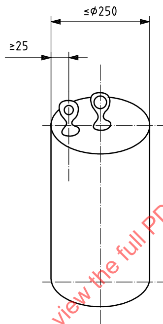
Figure 6 — Rigid steel mass
