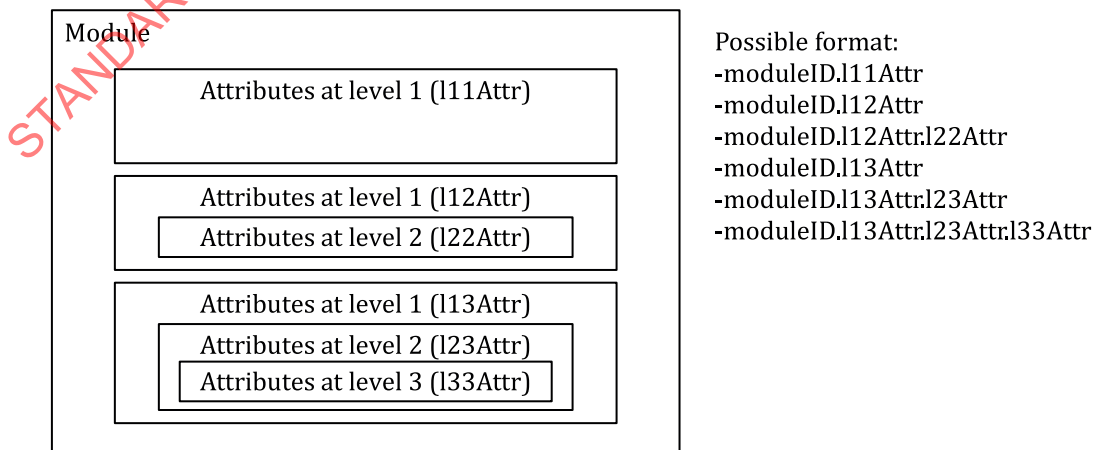
Figure A.1 — Relationships of a module and attributes in each level
