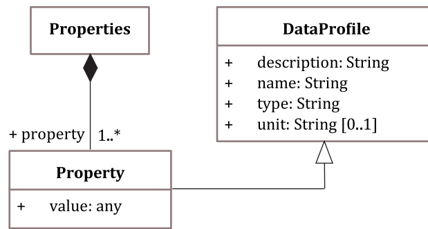
Figure 4.6 — Class diagram for class Properties
