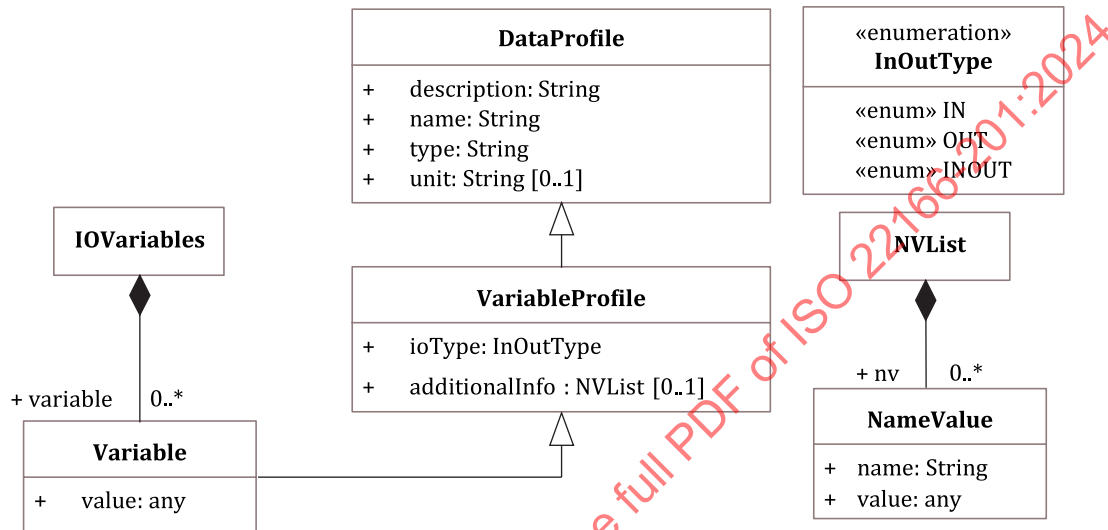
Figure 4.7 — Relationships between classes for class IOVariables
