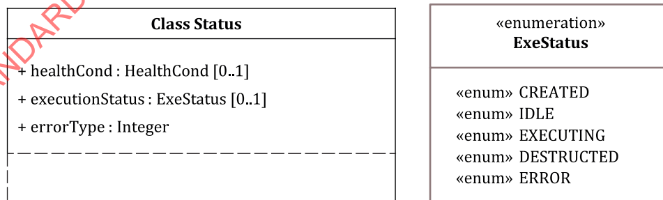
Figure 4.8 — Class diagram for class Status
