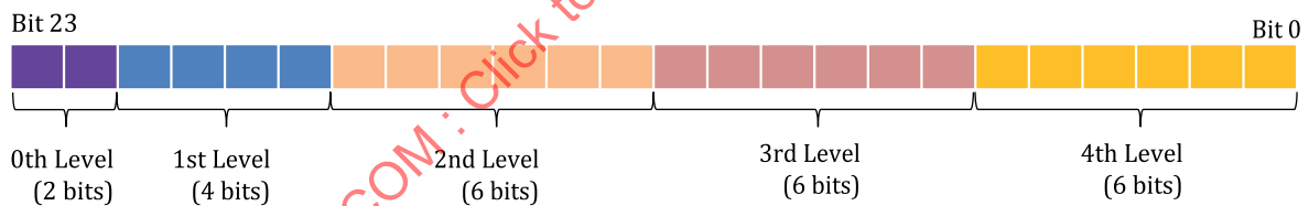
Figure B.2 — Fields for CategoryID
