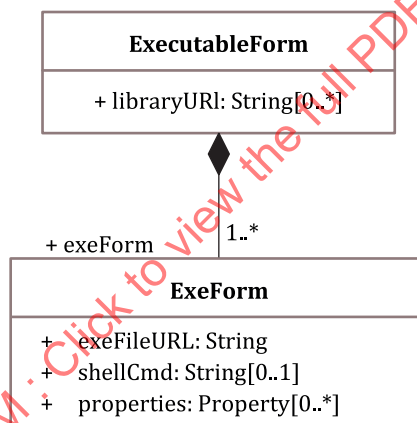
Figure 4.13 — Relationship between classes for class ExecutableForm
