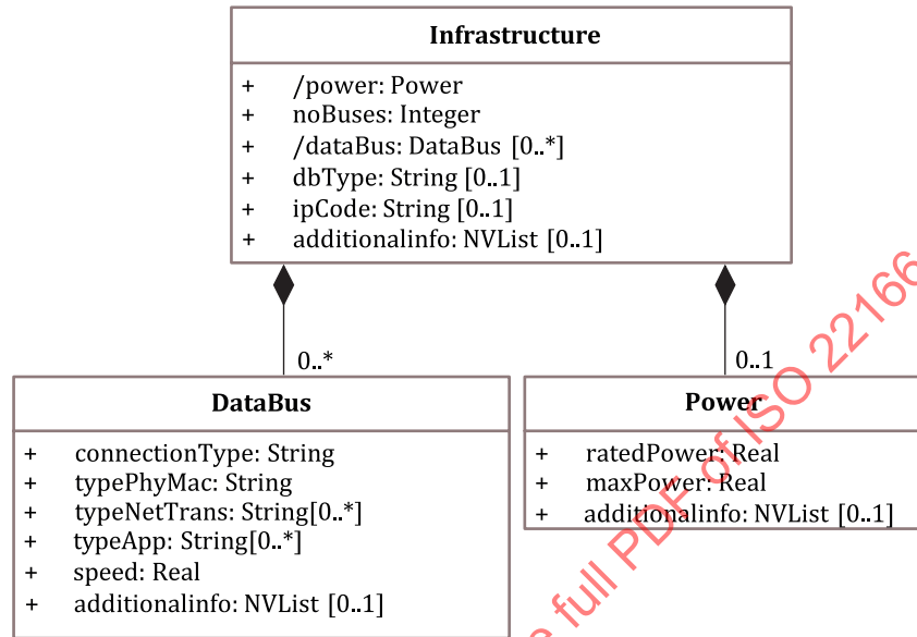
Figure 4.10 — Relationships between classes for class Infrastructure
