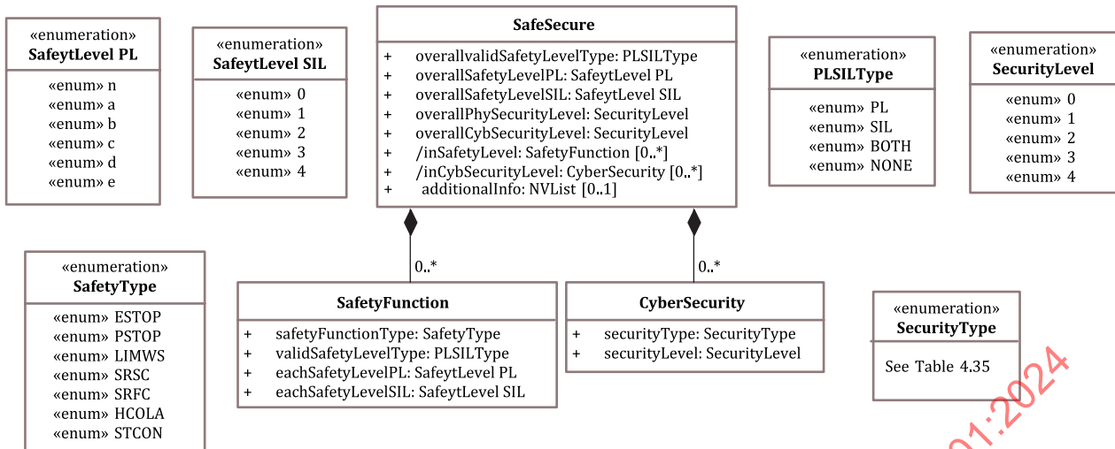
Figure 4.11 — Relationships between classes for class SafeSecure
