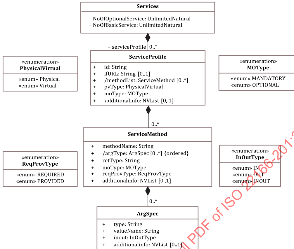
Figure 4.9 — Relationships between classes for class Services
