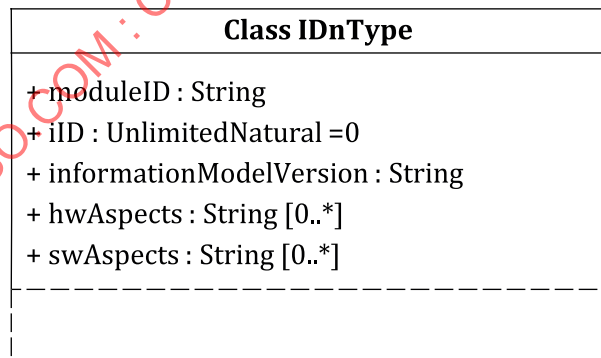
Figure 4.5 — Class diagram of class IDnType
