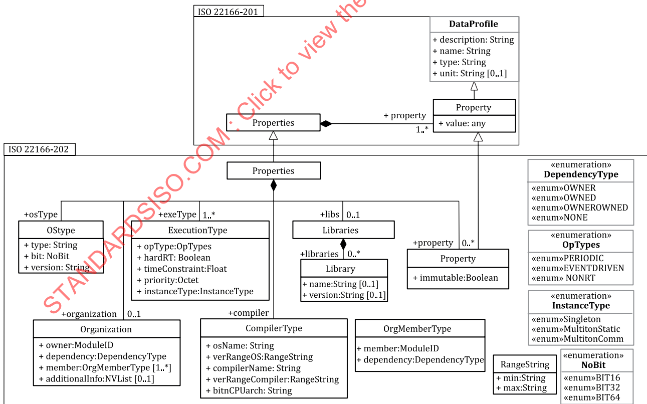
Figure 6 — Relationships between classes for class Properties
