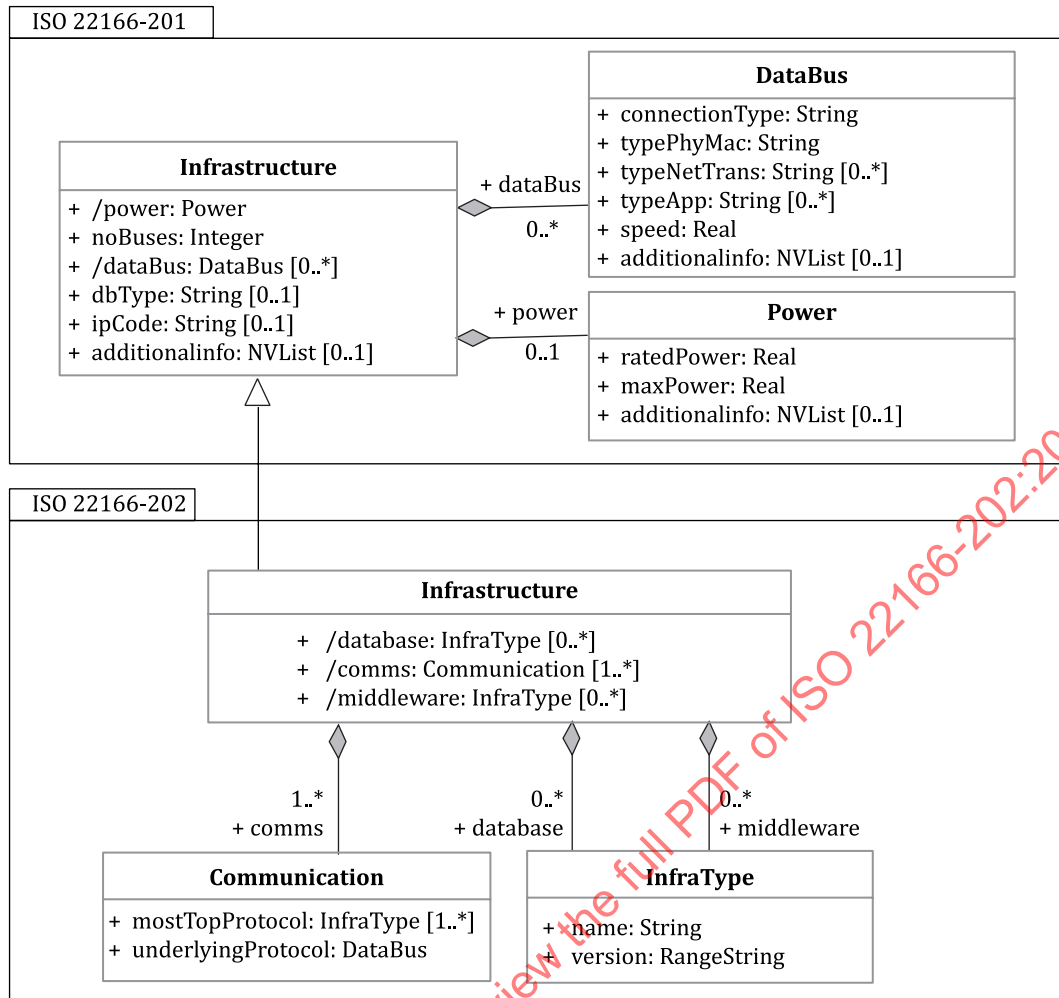
Figure 10 — Relationships between classes for class Infrastructure
