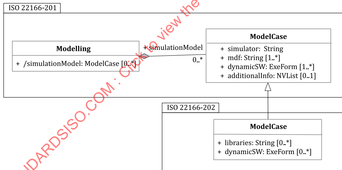
Figure 11 — Relationship between classes for class Modelling
