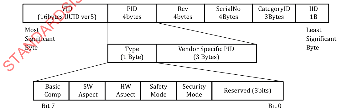
Figure A.1 — Data types of elements of a module ID
