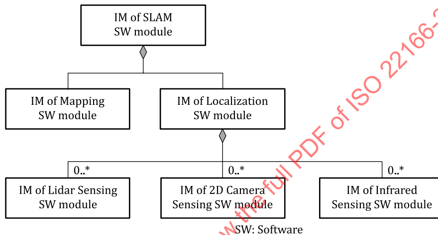
Figure C.1 — Example of information models for a SLAM software module
