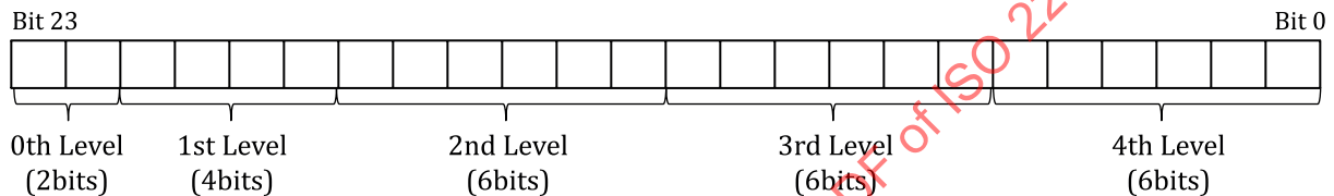
Figure A.2 — Fields of CategoryID
