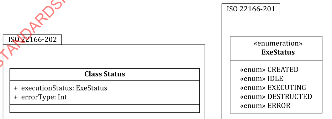
Figure 8 — Class diagram of class Status
