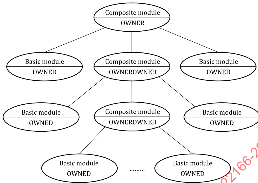
Figure 5 — Example diagram of composite module with dependency type
