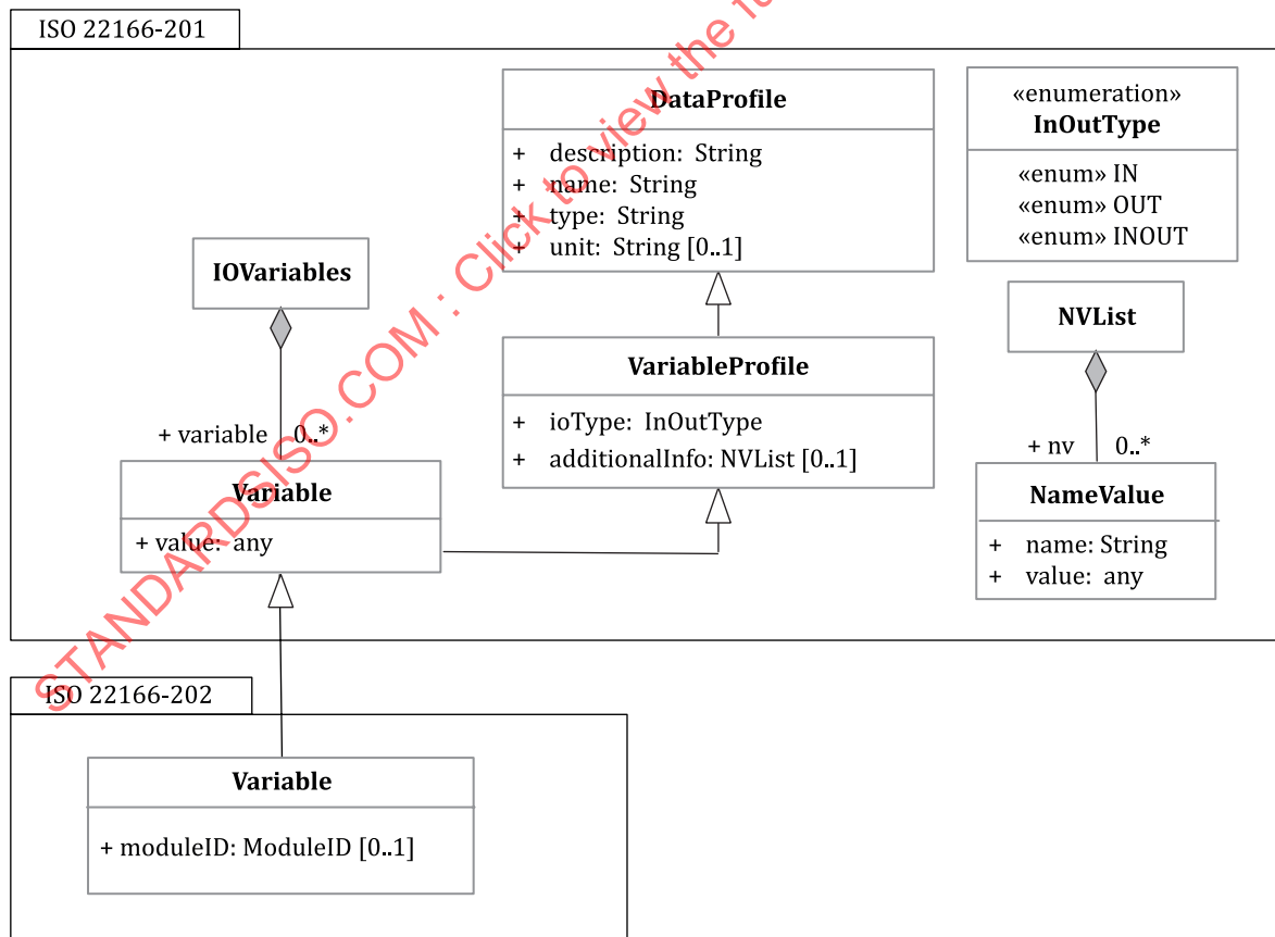
Figure 7 — Relationships between classes for class IOVariables
