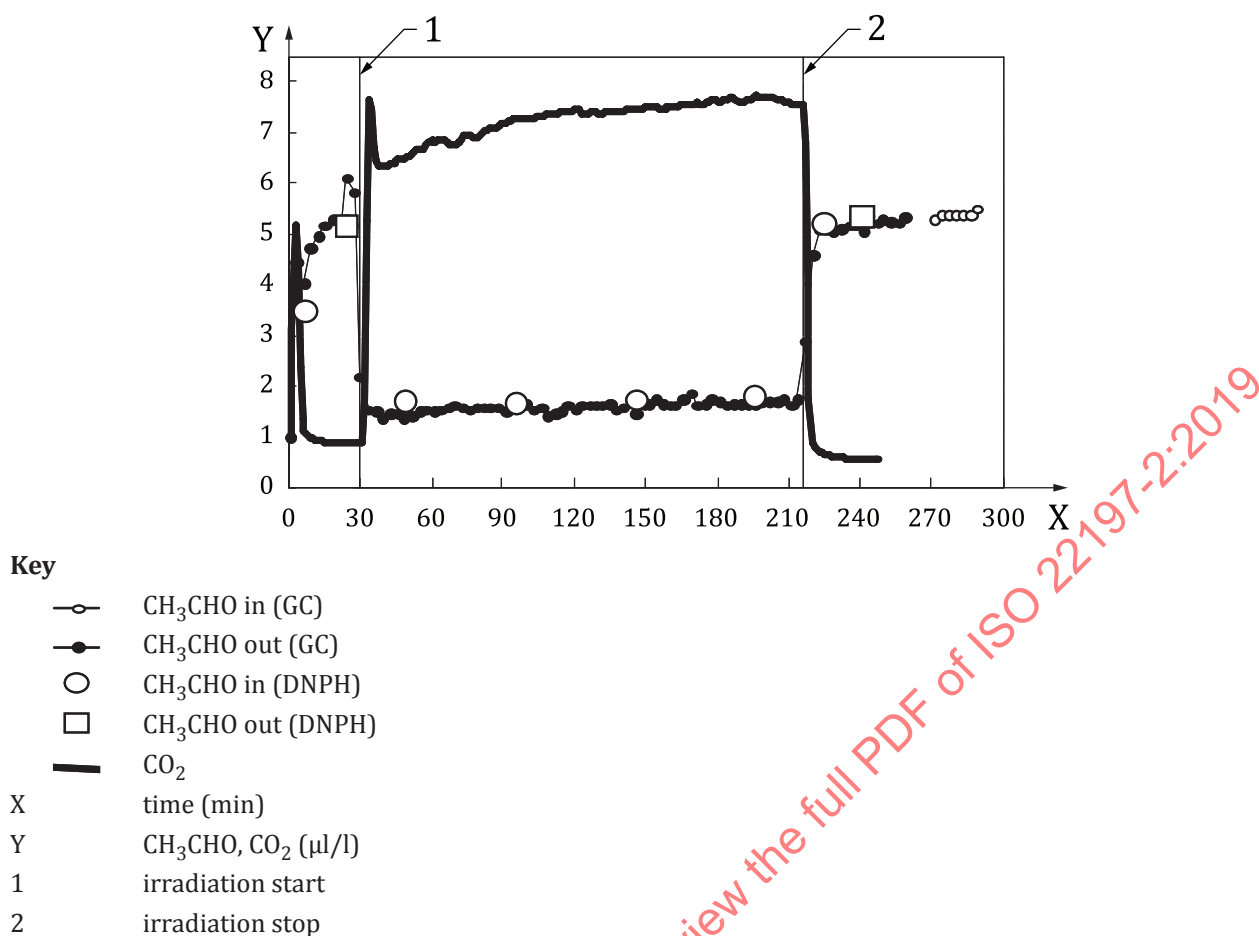
Figure 4 — Typical trace of acetaldehyde and CO 2 concentration during the test operation
