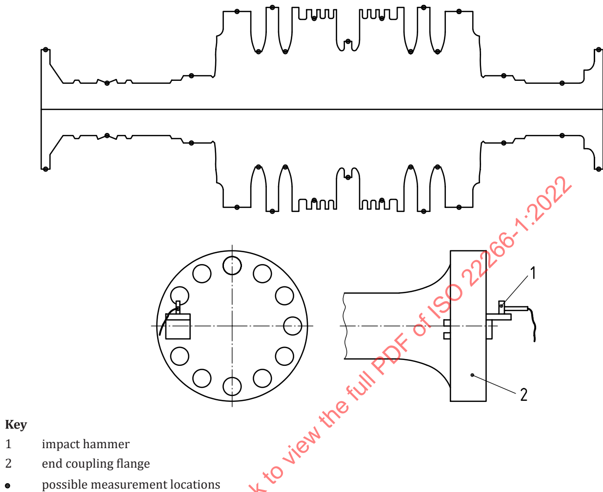
Figure A.5 — Factory test under standstill condition
