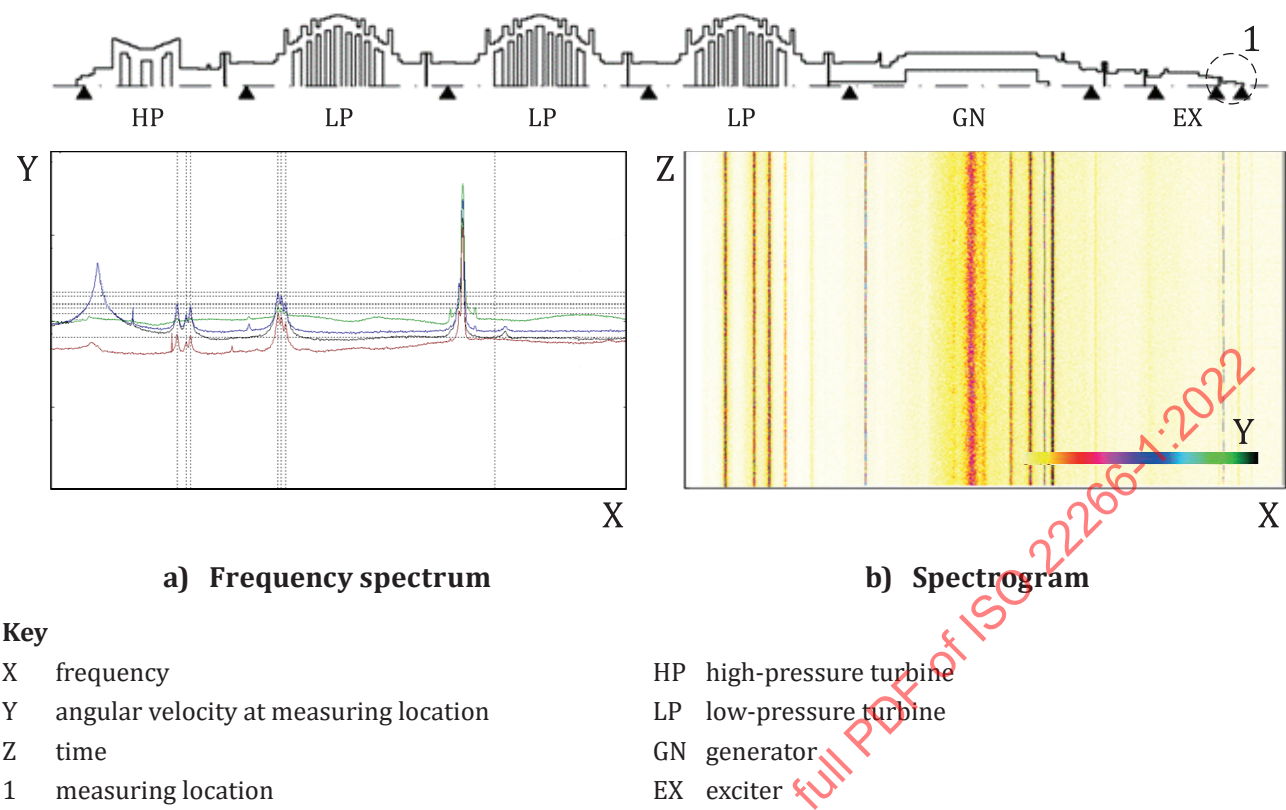
Figure A.7 — Example of an on-site torsional test set up
