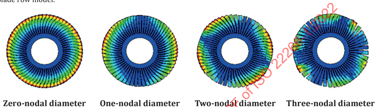
Figure 2 — Schematic illustration of different nodal diameters
