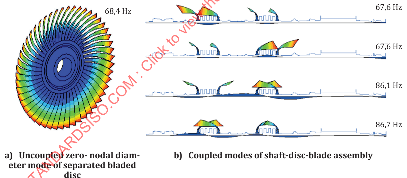
Figure 2 — Schematic illustration of different nodal diameters
