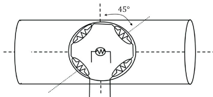
Figure A.4 — Measurement with magnetostrictive sensor
