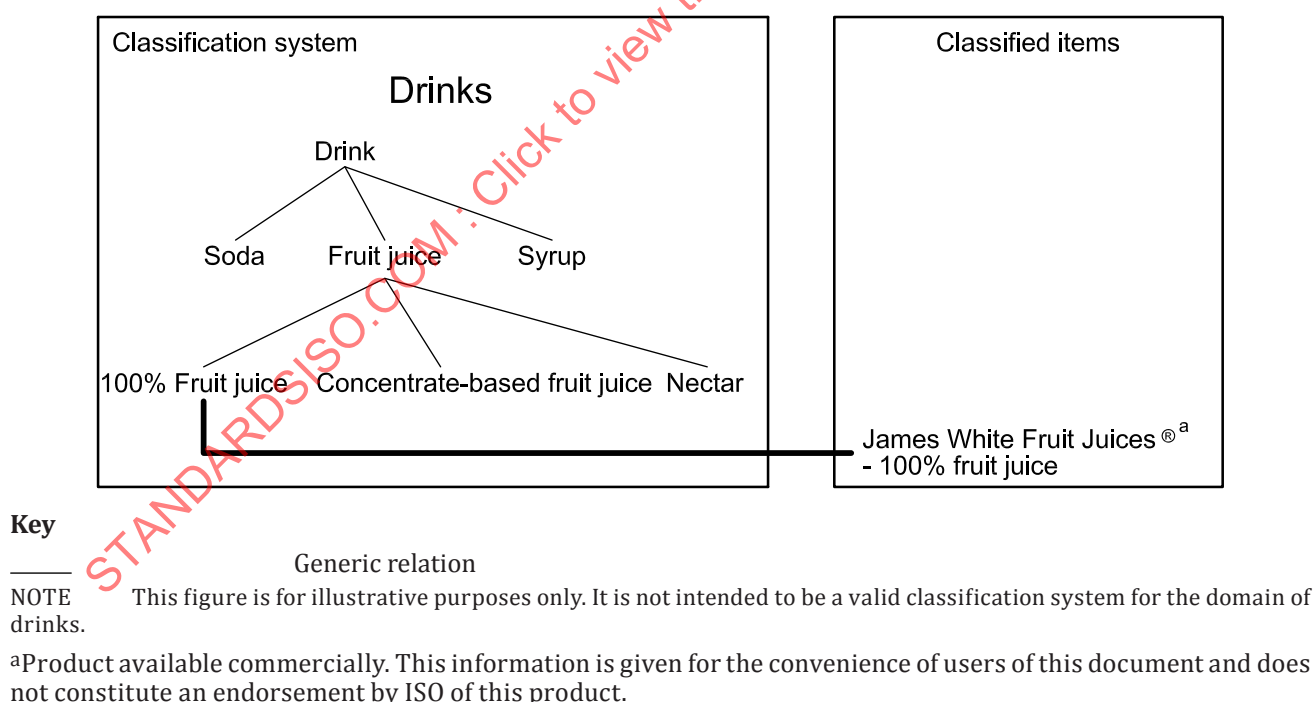
Figure 2 — Example of an enumerative classification system
