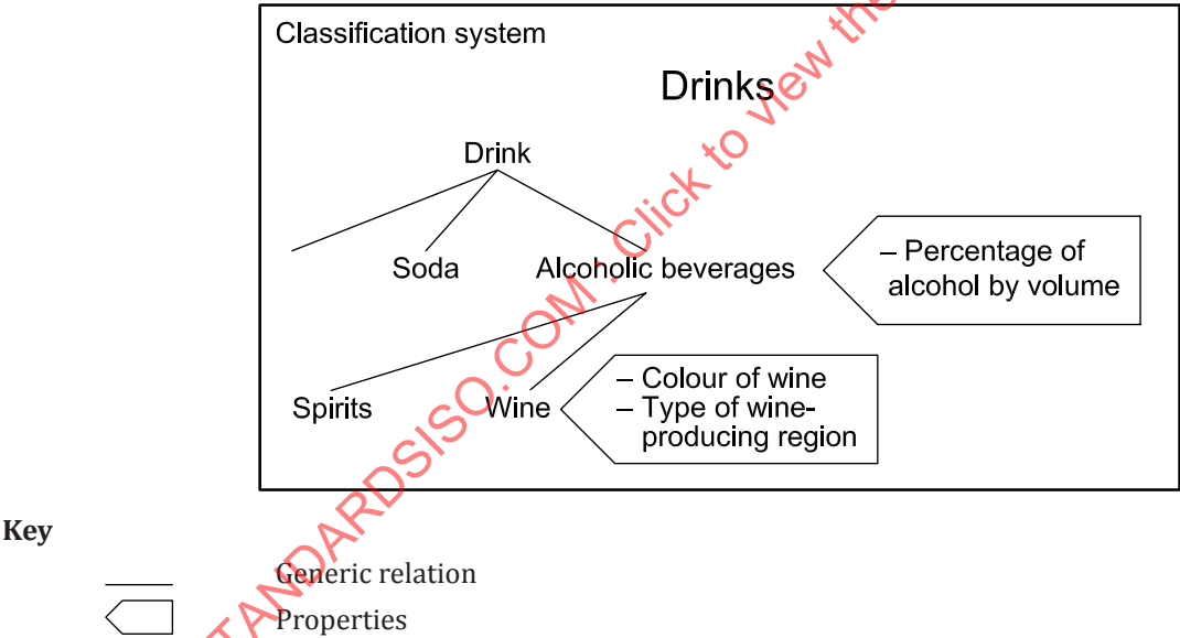
Figure 7 — Classification system with properties allowed at any class
