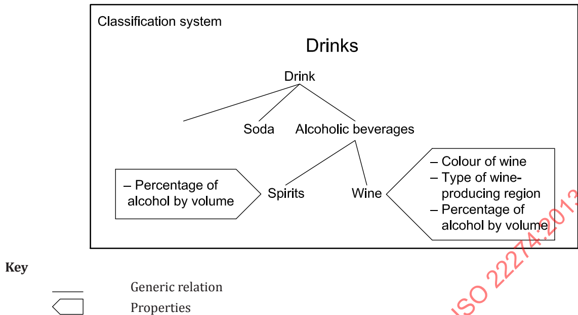
Figure 8 — Classification system with properties allowed only at leaf classes
