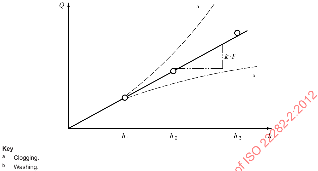
Figure B.2 — Infiltrated water amount depending on the pressure difference
