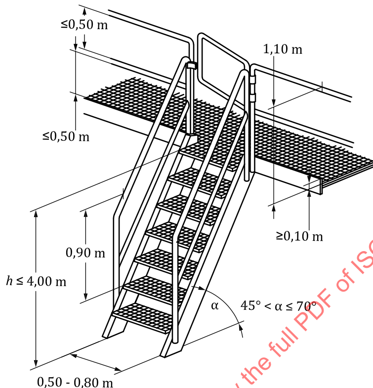
Figure 1 — Access stairs type 2
