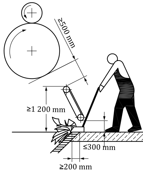
Figure 3 — Protection against falling from a height on recovery pulper under the winder
