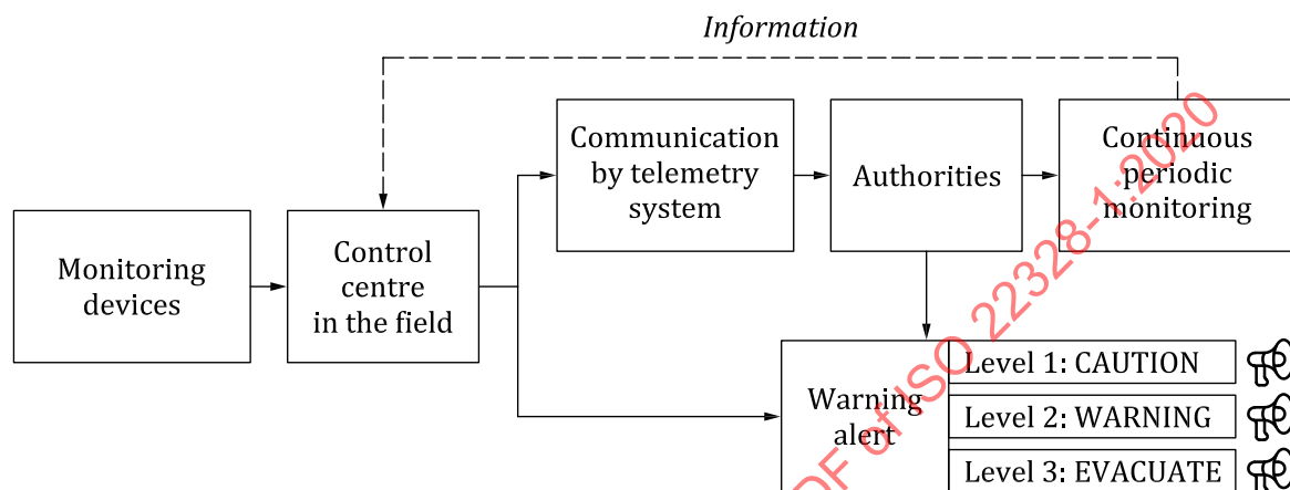
Figure C.1 — Example of a scheme of a community-based early warning system
