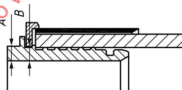
Figure A.2 — Examples of an axial press fitting
