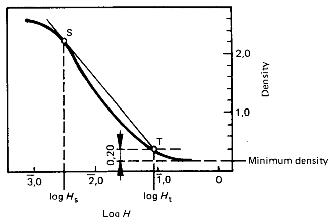
FIGURE — Curve of density against log H
