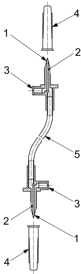
Figure 3 a) — Transfer set with an air inlet/air outlet
