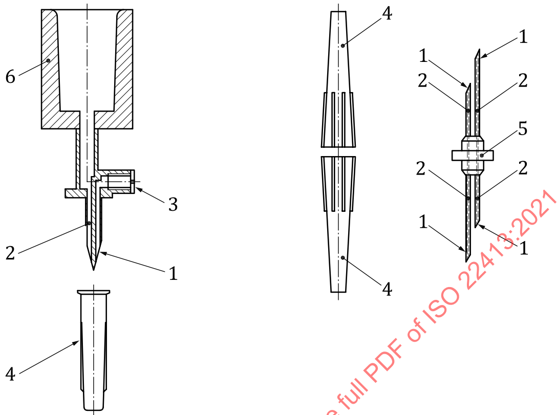
e) Transfer set with an air inlet/air outlet in combination with a small-bore connector
