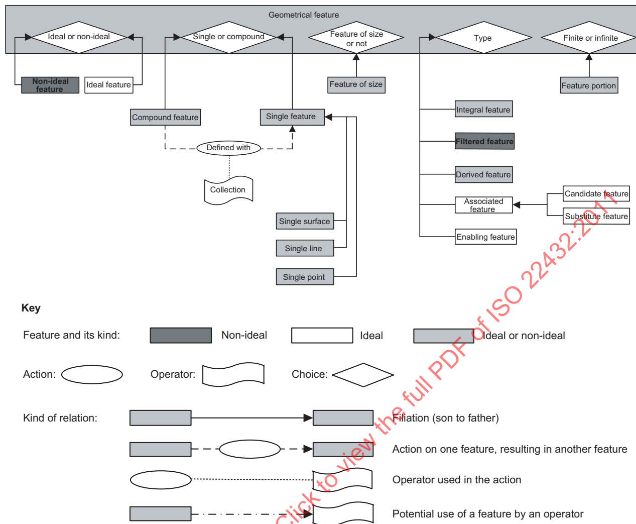
Figure A.2 — Attributes of a geometrical feature and types of feature
