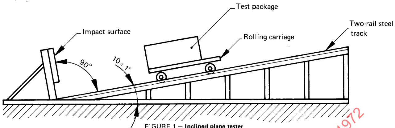
FIGURE 1 — Inclined plane tester
