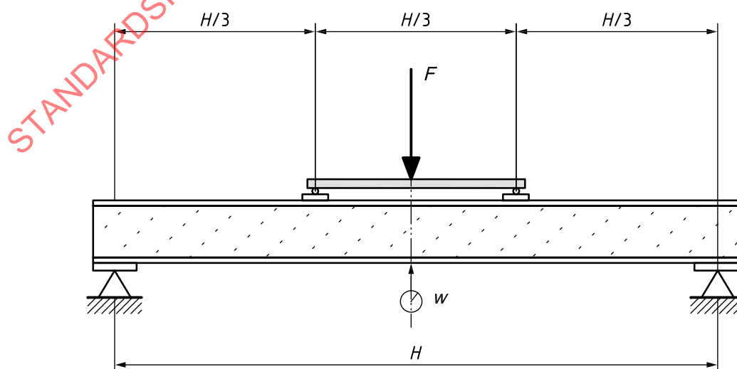
Figure 14 — General test set-up for out-of-plane bending
