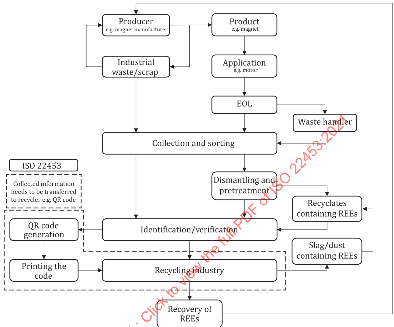
Figure 1 — Generic life cycle of REE recycling
