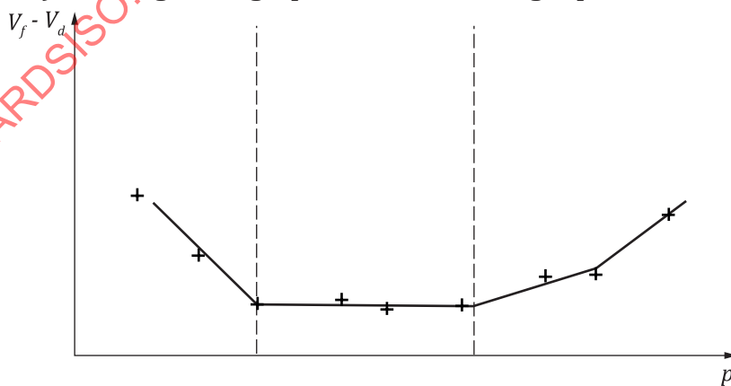
a) Shearing curve graph with shear strength parameters
