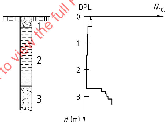
Figure D.9 — Dynamic probing in decomposed peat
