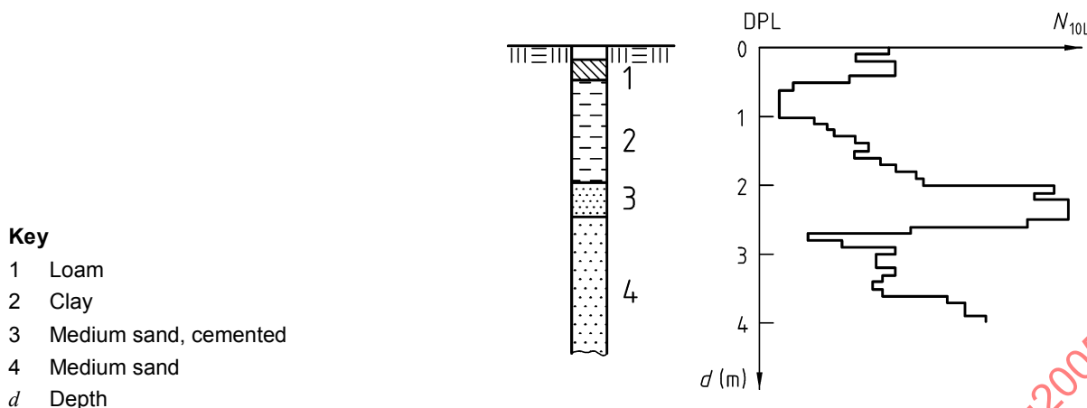
Figure D.4 — Increase in penetration resistance in a cemented medium sand
