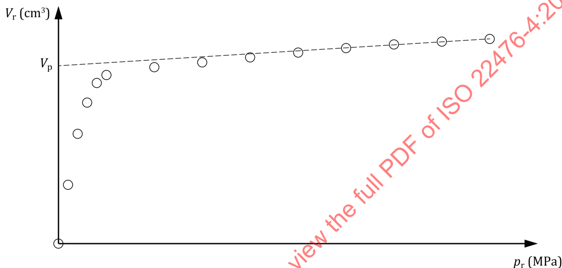
Figure B.2 — Volume loss calibration – Example
