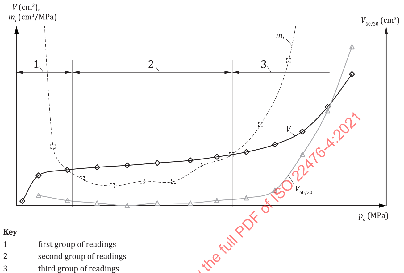
Figure D.3 — Pressuremeter test data points analysis – Example
