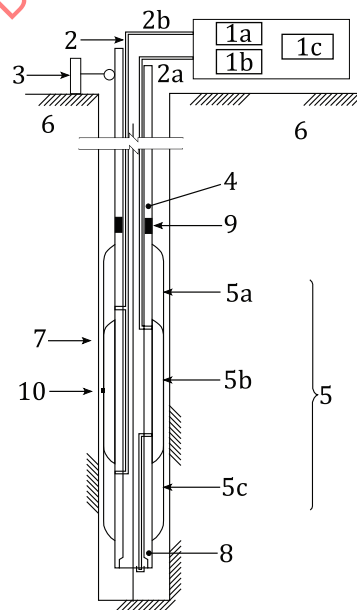
d) Tri-cell probe, with measurement of radial displacement
