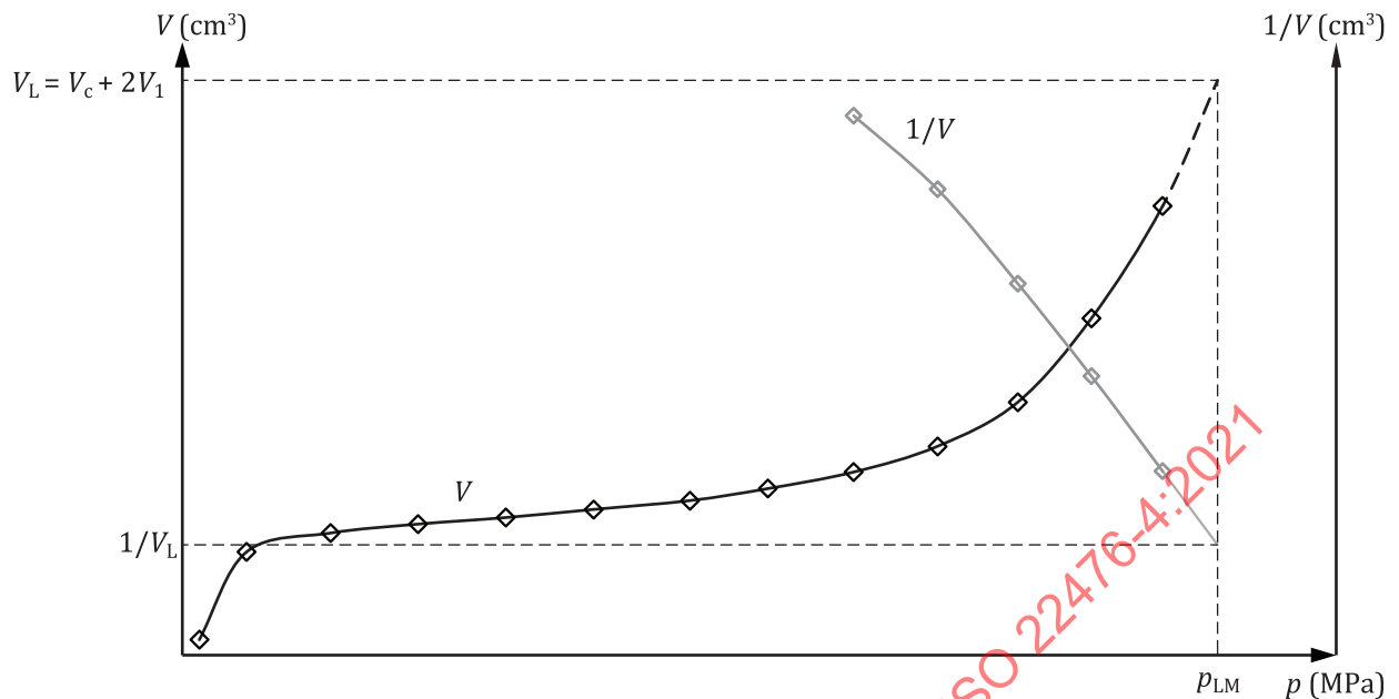
Figure D.5 — Ménard pressuremeter limit pressure, with reciprocal fitting and extrapolation method
