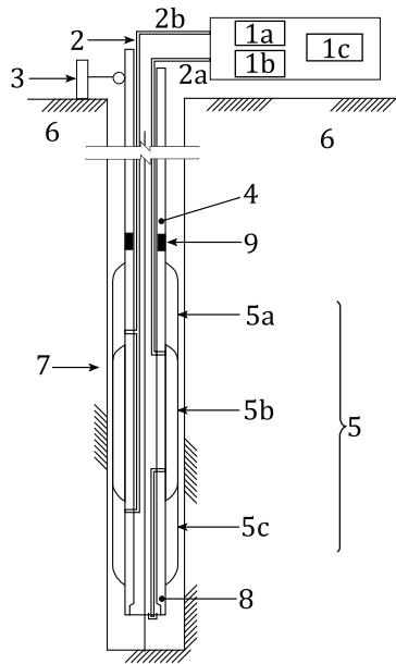
a) Tri-cell probe, G type, with measurement of volume of the measuring cell
