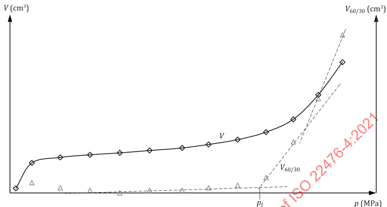
Figure D.4 — Pressuremeter creep pressure determination
