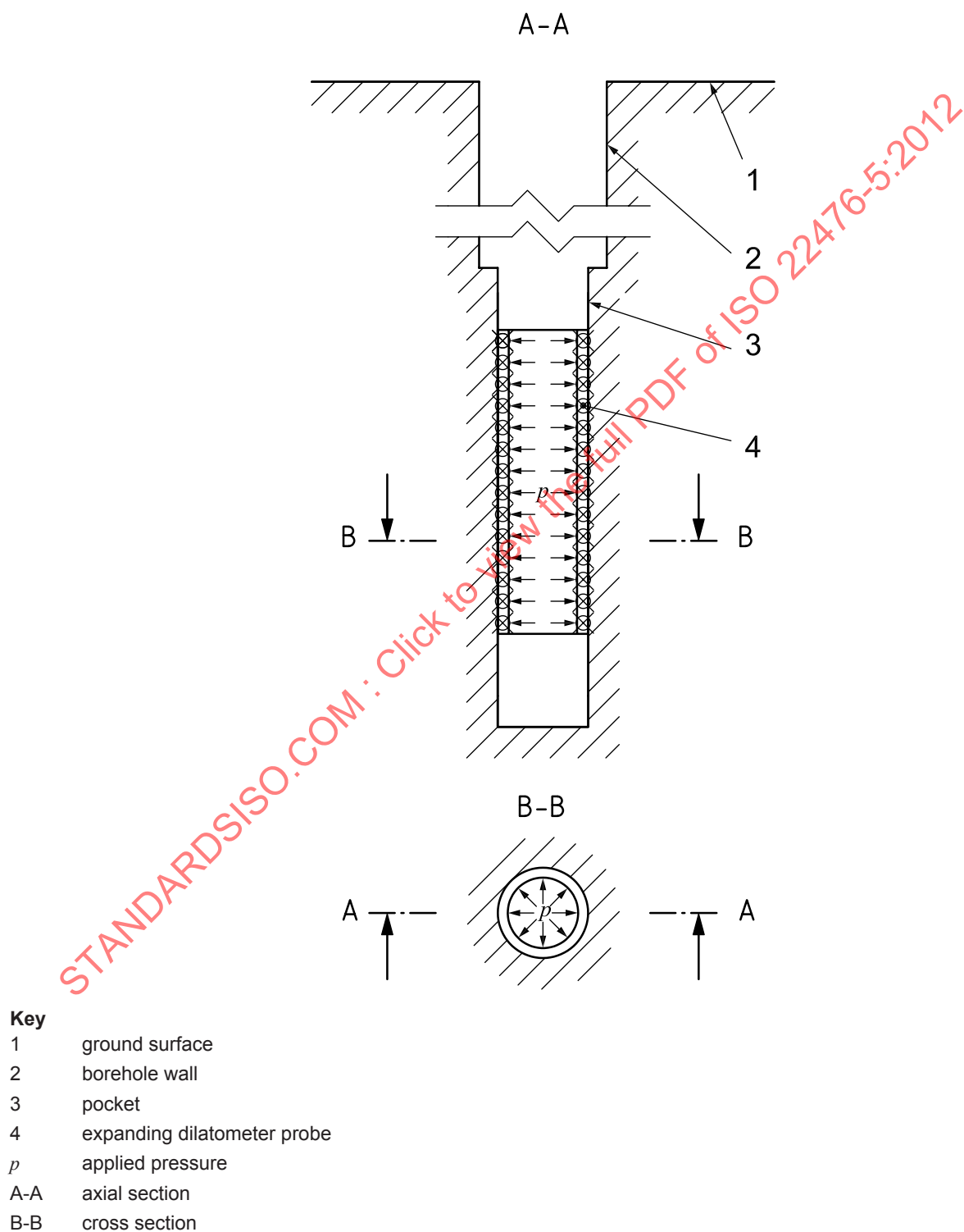
Figure 1 — Example of a flexible dilatometer test
