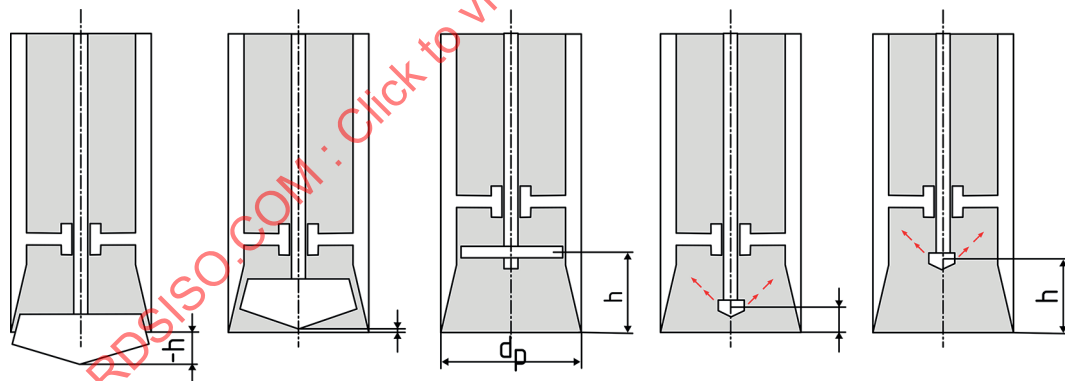
Figure 4 — Distance between the cutting tool and the cutting edge
