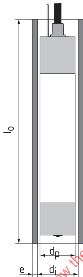
Figure A.2 — Compression calibration cylinder for the self-boring pressuremeter
