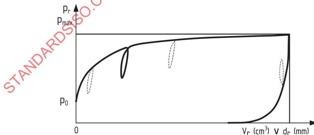
Figure 7 — Example of a self-boring pressuremeter test result
