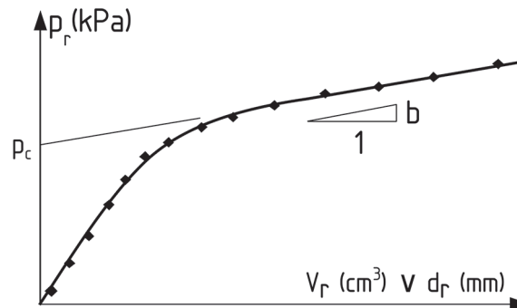
Figure A.1 — Stiffness plots for the self-boring pressuremeter
