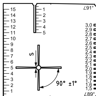
Figure C.1 — Example of the mould for vane requirements and dimension checks where dimensions are in centimetres and angles in degrees
