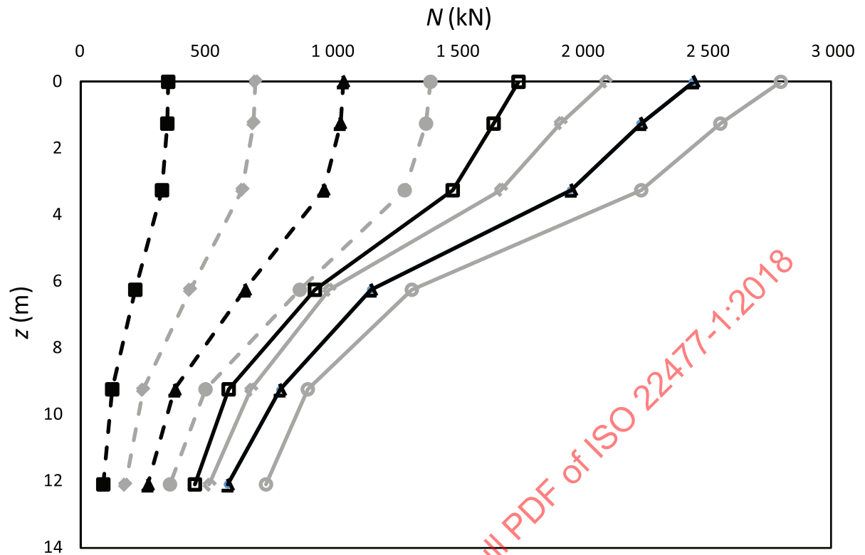
Figure 10 — Axial force–depth ( N - z ) plot
