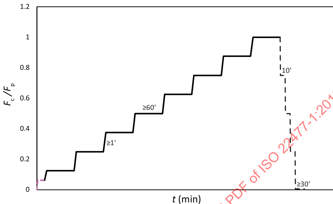
Figure 3 — Load step sequence for one cycle procedure
