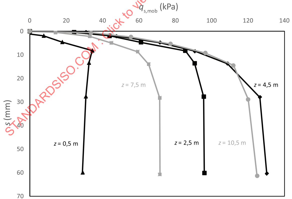
Figure 11 — Unit shaft friction mobilisation ( q_{s,mob} - s ) plot
