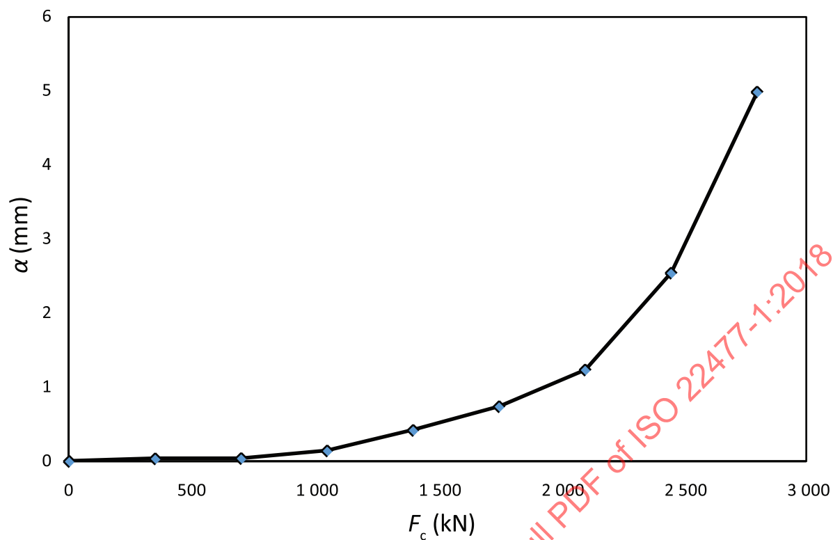
Figure 8 — Load-creep rate ( F_c - \alpha ) plot
