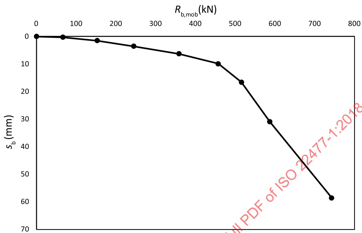
Figure 12 — Mobilised base resistance-base settlement ( R_{b,mob} - s_b ) plot
