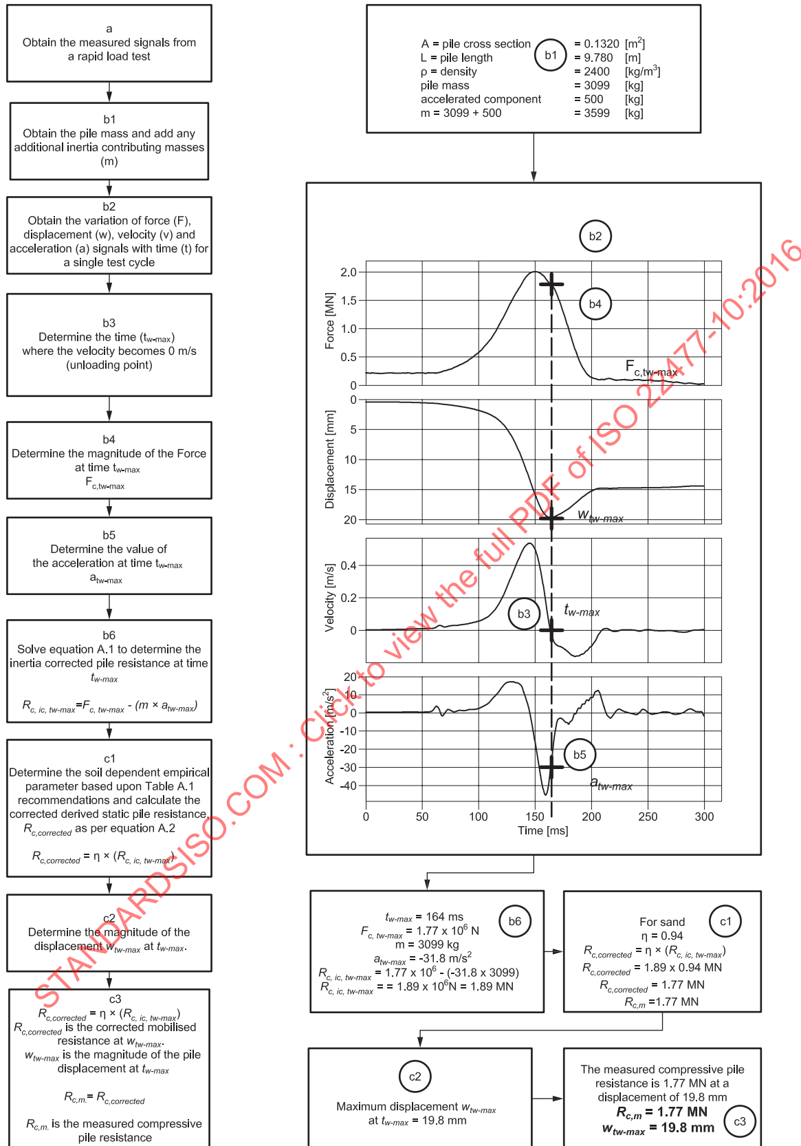
Figure A.2 — Analysis process for a single cycle using example data and calculation of R_{c, m}
