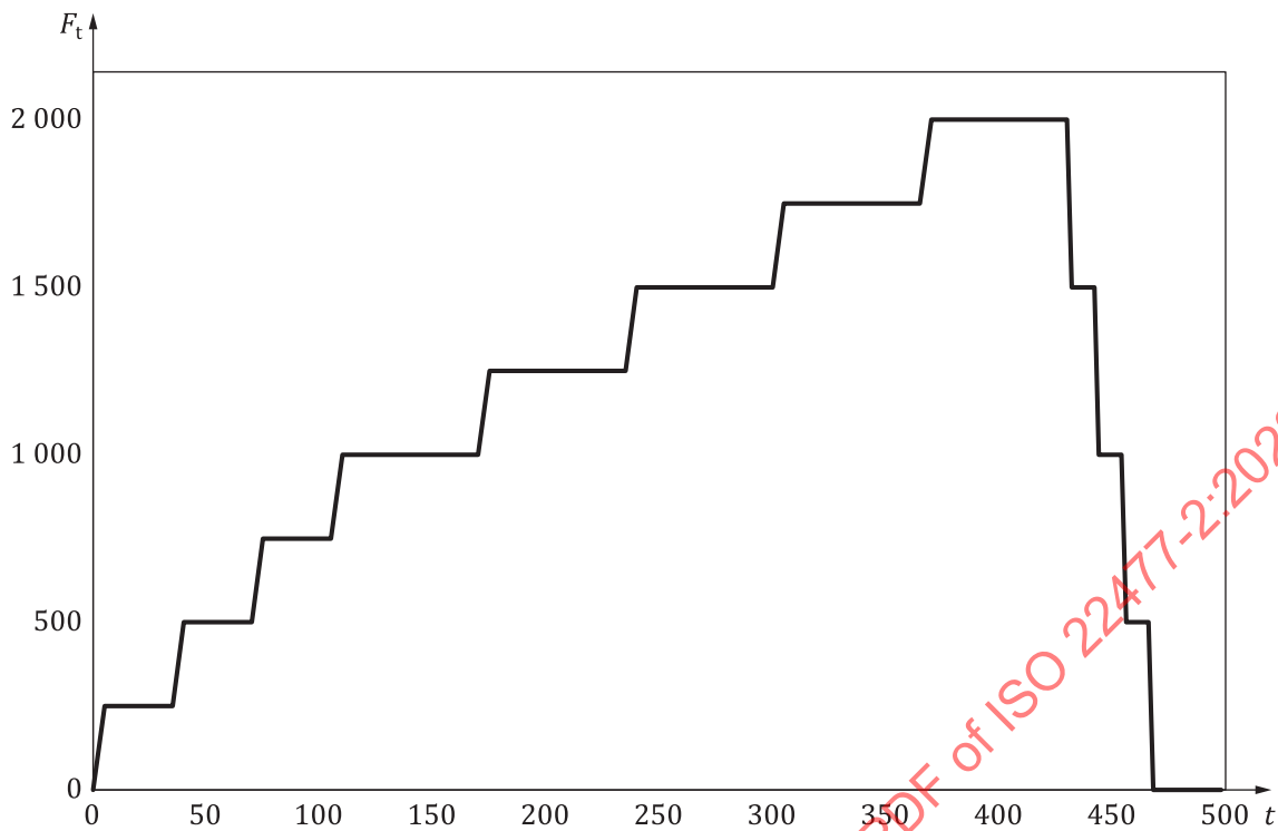
Figure 5 — Time-load ( t - F_t ) plot
