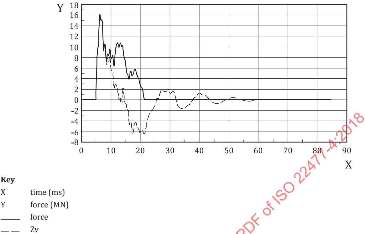
Figure B.4 — Time history for impact force and velocity multiplied by the impedance at pile top
