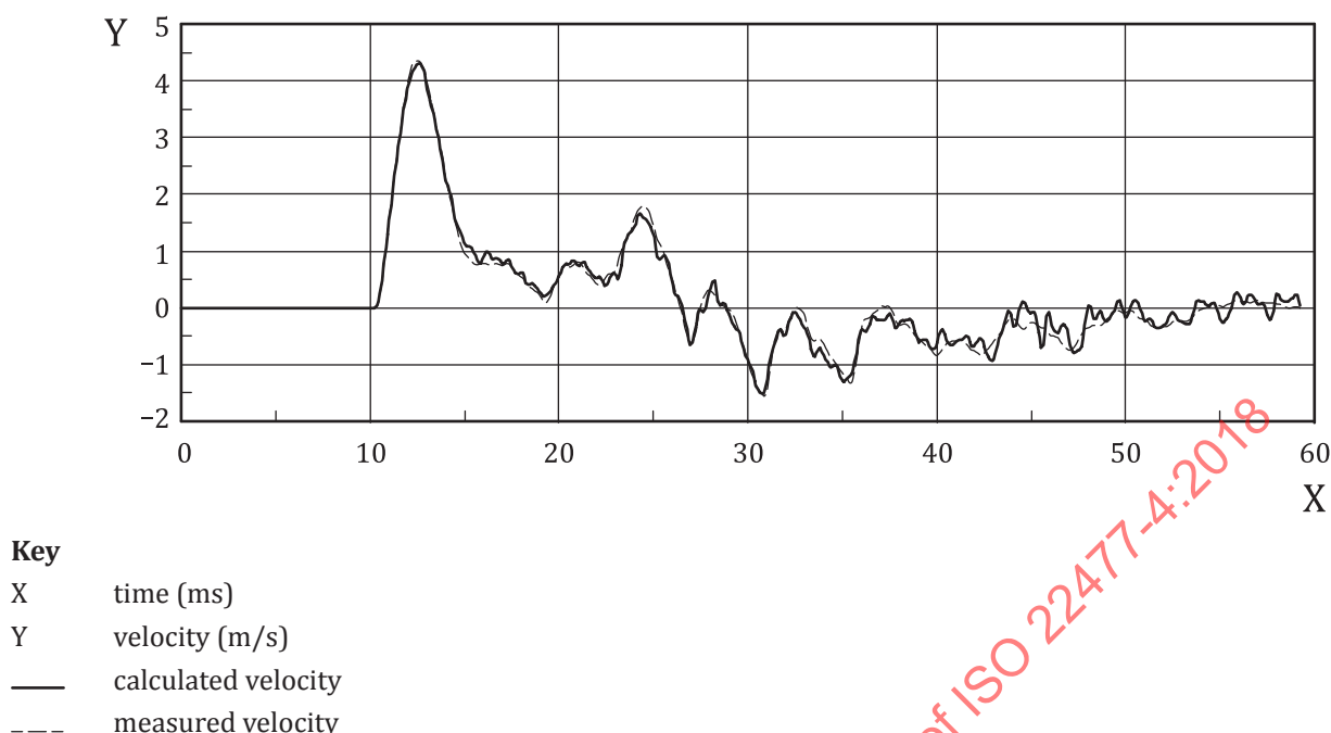
Figure E.5 — Comparison of the recorded pile velocity and the pile velocity calculated using the model
