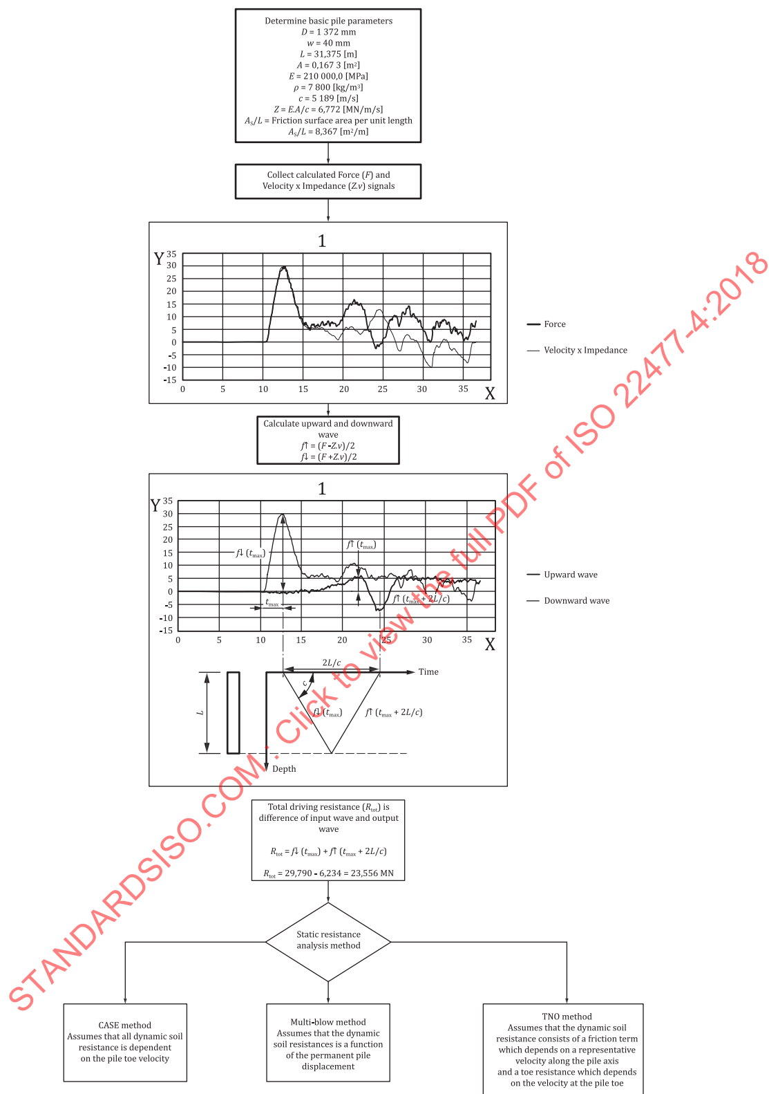
Figure D.2 — Flowchart showing the general approach to closed form analysis of a dynamic test
