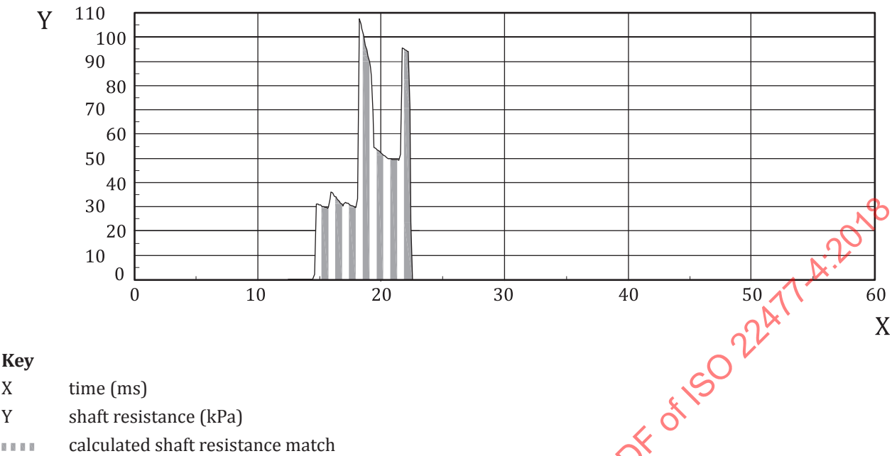
Figure E.6 — Result of signal matching process showing shaft resistance distribution as a function of time
