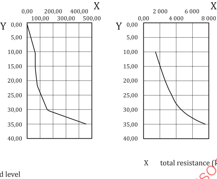
Figure B.10 — Derived driving record match of compressive resistances
