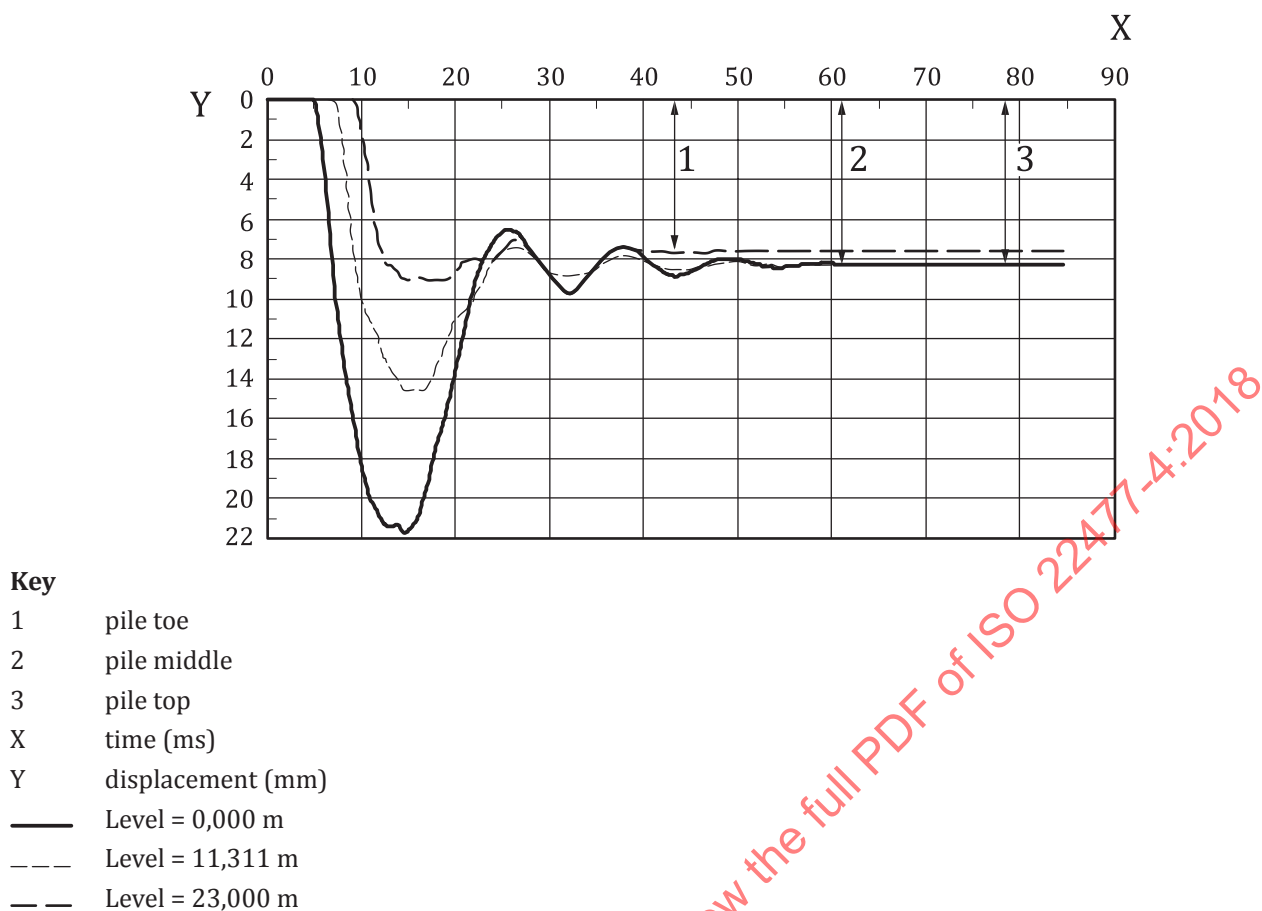
Figure B.6 — Determination of permanent set for a hammer blow
