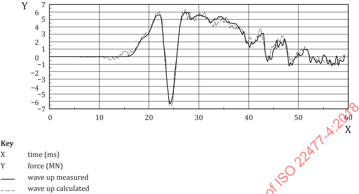
Figure E.3 — Comparison of the measured wave up and the wave up calculated based upon the measured wave down time history using the pile-soil-model
