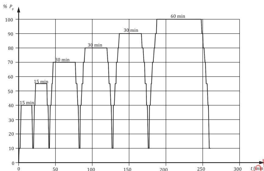
Figure 9 — Loading sequence for investigation test for coarse soil and rock
