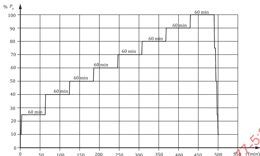
Figure 19 — Loading sequence for investigation test
