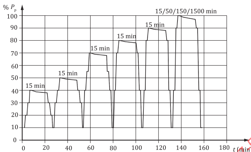
Figure 16 — Loading sequence for investigation test
