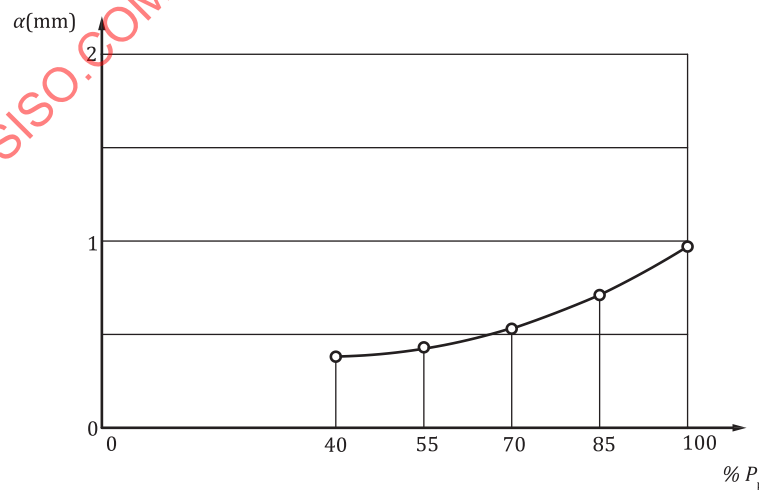
Figure 14 — Plot of \alpha versus anchor load, example suitability test
