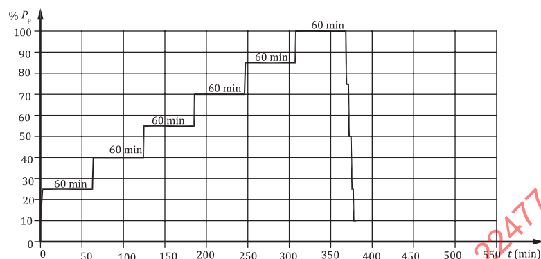
Figure 21 — Loading sequence for suitability test
