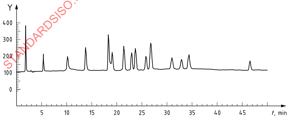
c) Detection at 254 nm
