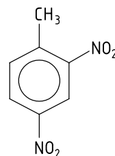
2,4-Dinitrotoluene
