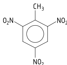
2,4,6-Trinitrotoluene (TNT)
