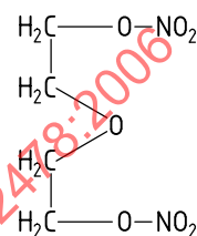
Diethylene glycol dinitrate (DEGN)
