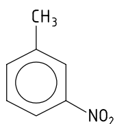
3-Nitrotoluene
