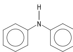
Diphenylamine (DPA)
