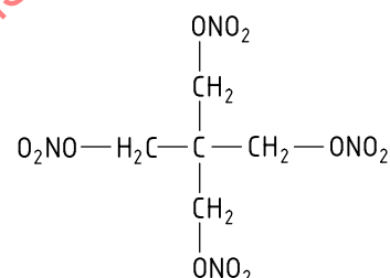
Nitropenta (PETN)
