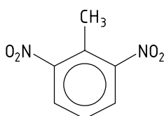
2,6-Dinitrotoluene
