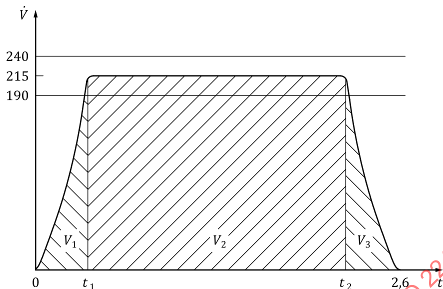
Figure 1 — Puff profile (idealized)
